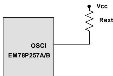
Fig. 21 Circuit for Internal C Oscillator Mode
