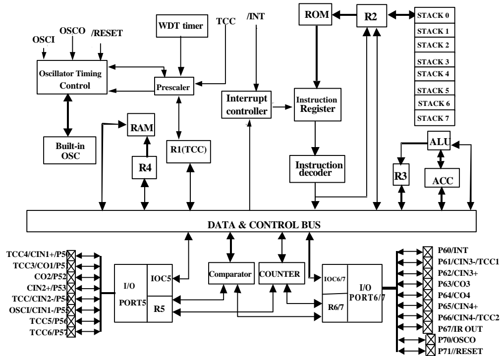
Fig. 3 Functional block diagram
