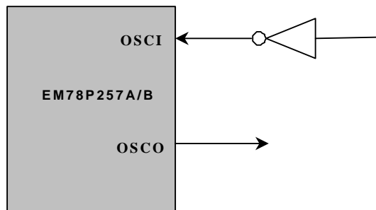
Fig. 18 Circuit for External Clock Input
