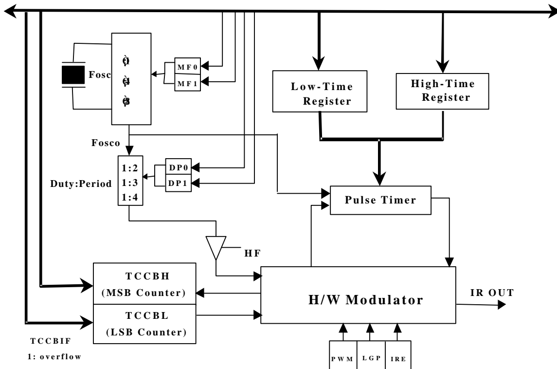
Fig. 27 Hardware Modulator
