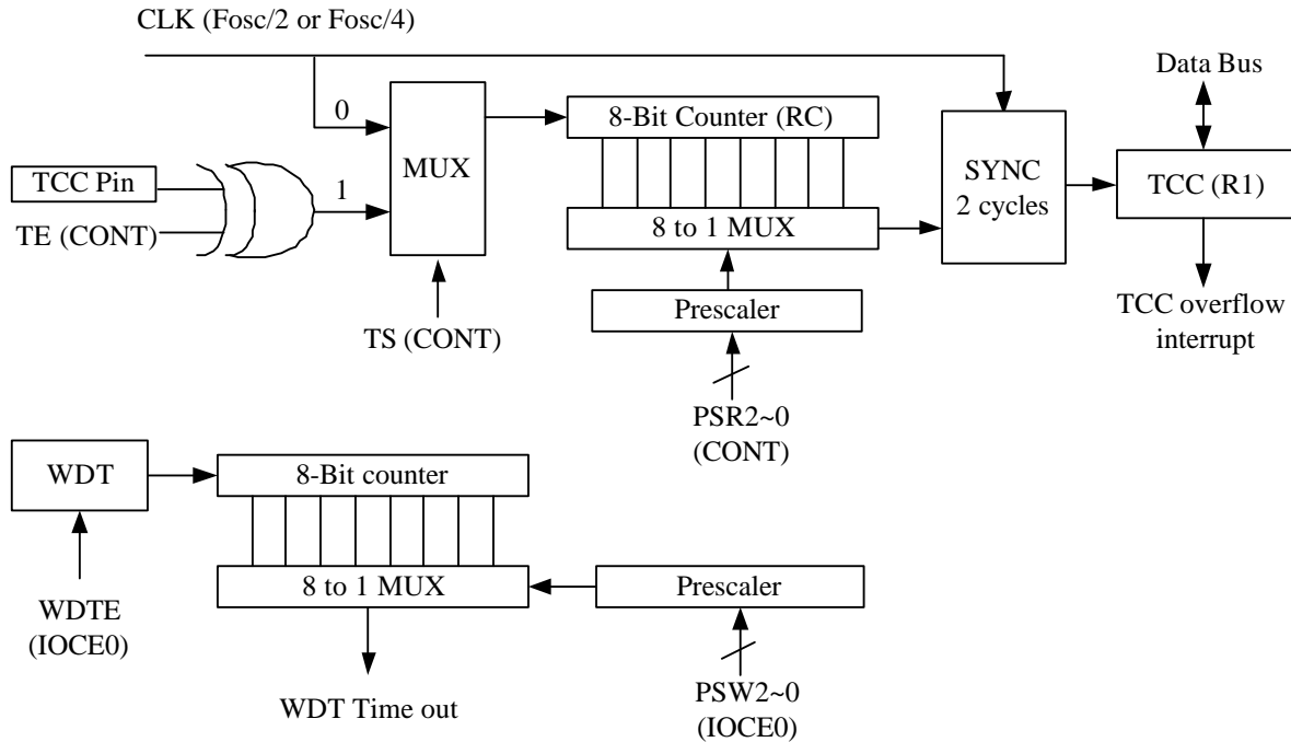
Fig. 6 Block Diagram of TCC and WDT
