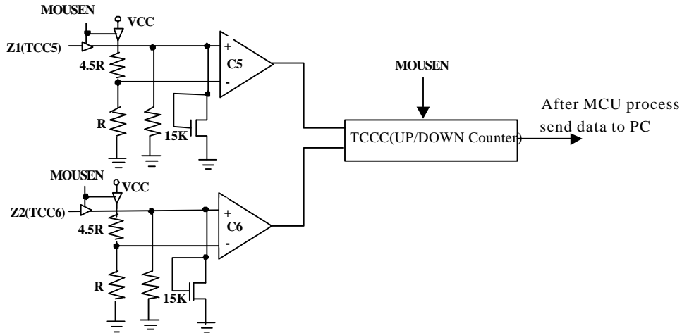
Fig. 25 Mouse Function Diagram
