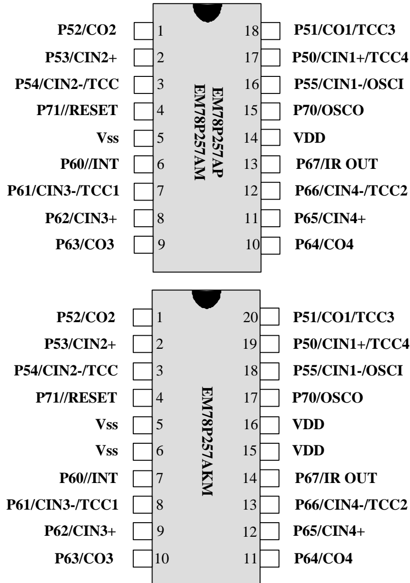
Fig. 1 Pin Assignment - EM78P257AP/AM/AKM
