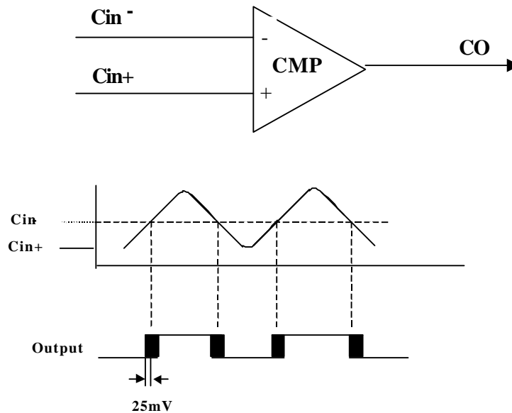
Fig. 16 Comparator Operating Modes
