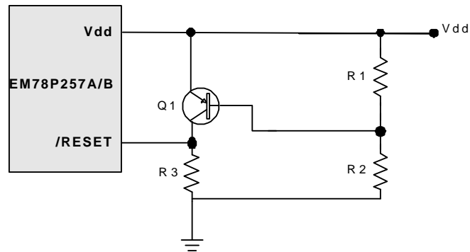
Fig. 24 Circuit 2 for the residue voltage protection
