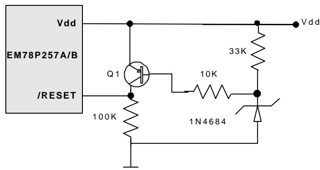
Fig. 23 Circuit 1 for the residue voltage protection
