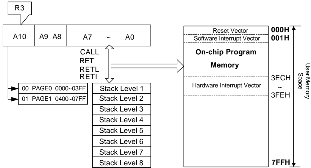
Fig. 4 Program counter organization
