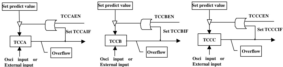
Fig. 14 TIMER Block Diagram
