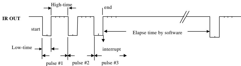
Fig. 26 Example Pulse Train Output of IR OUT Pin
