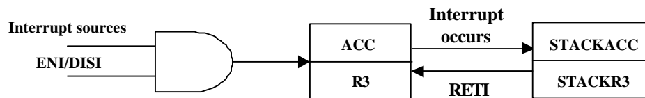
Fig. 12 Interrupt input circuit
