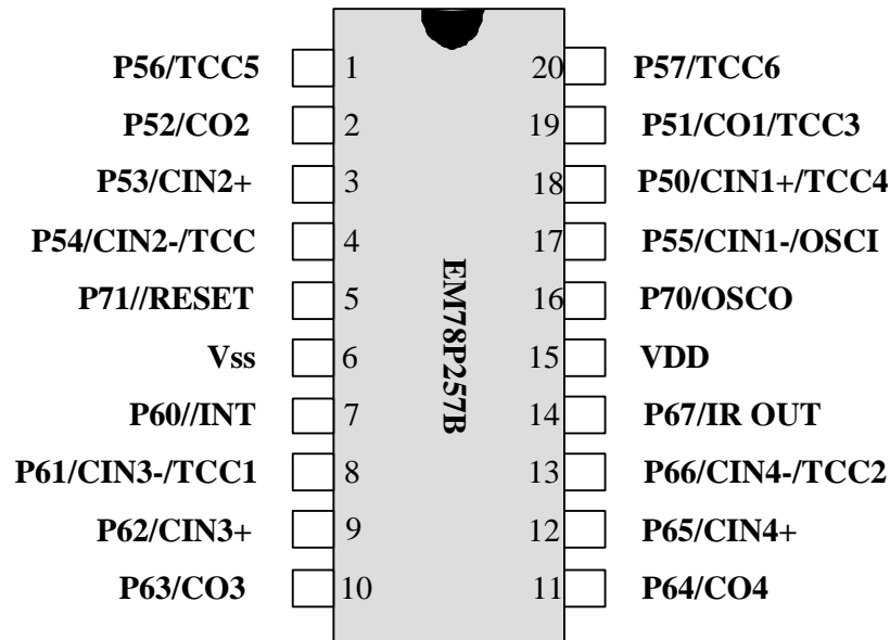
Fig. 2 Pin Assignment - EM78P257BP/BM
