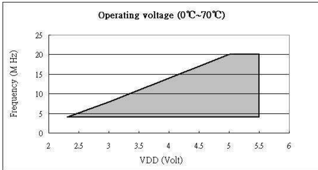
Fig. 49 Operating voltage under temperature range of 0°C to 70°C
