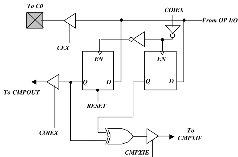
Fig. 17 The Output Configuration of a Comparator
