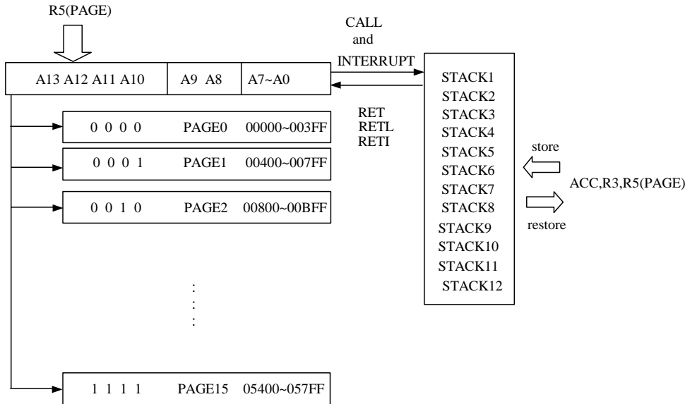
Fig.3 Program counter organization
