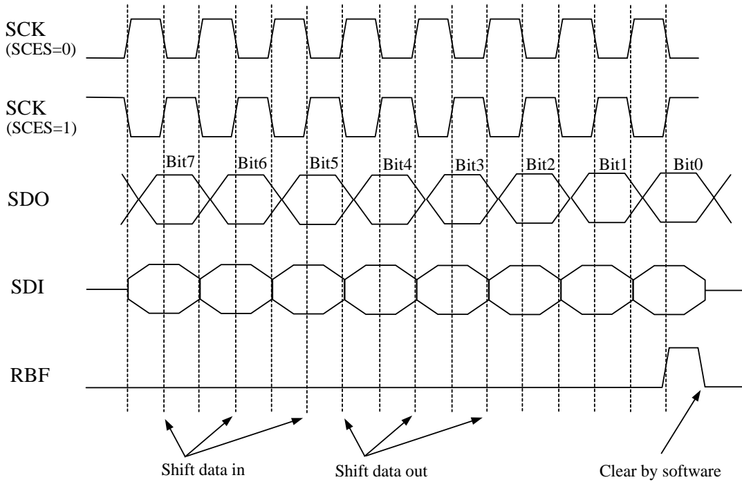
Fig.6 SPI timing
