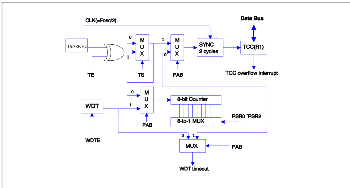
Fig.8 Block diagram of TCC WDT
