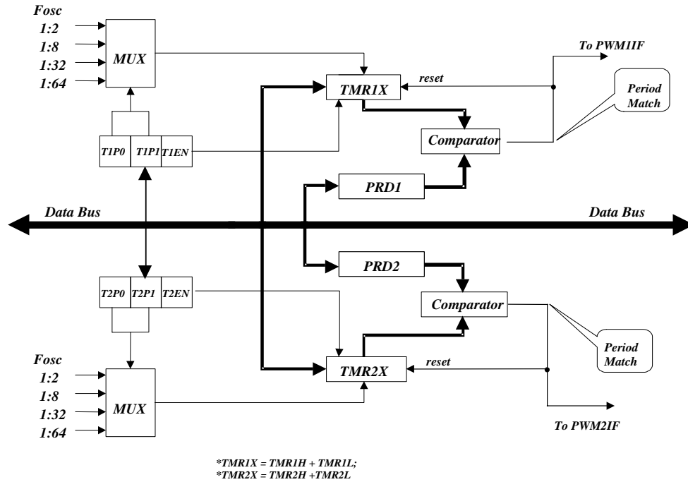
Fig.14 TMRX Block Diagram
