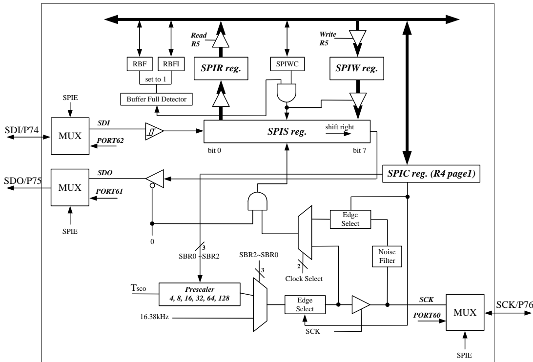
Fig.5 SPI structure
