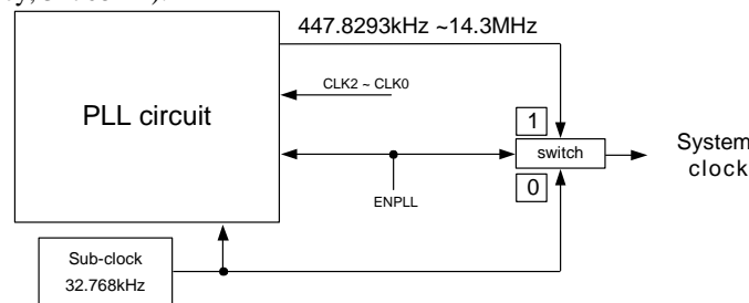
Fig.7 The relation between 32.768kHz and PLL
