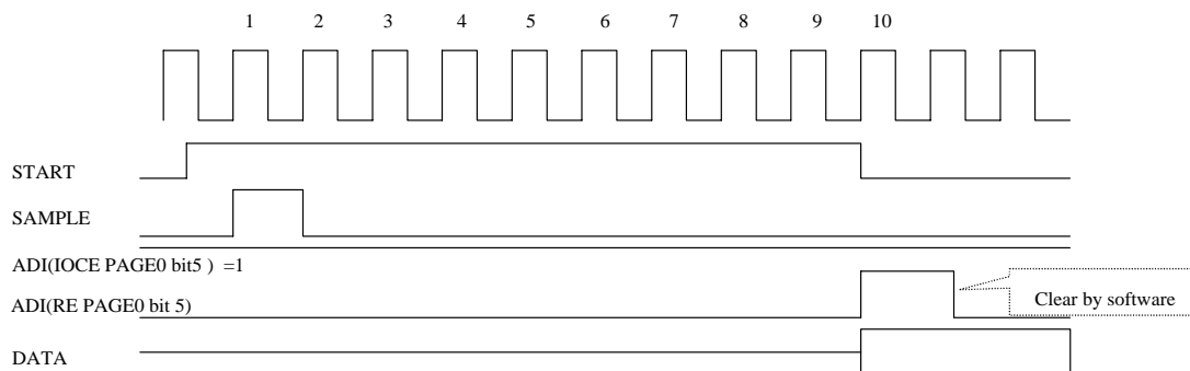
Fig.10 A/D converter timing
