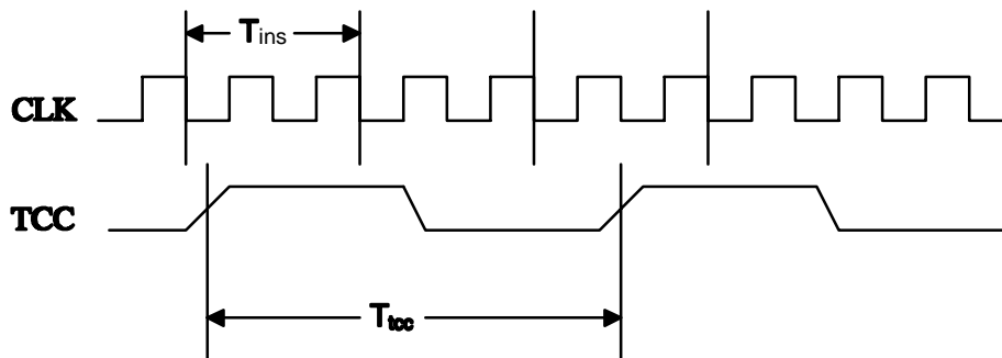
Fig.17 AC timing
