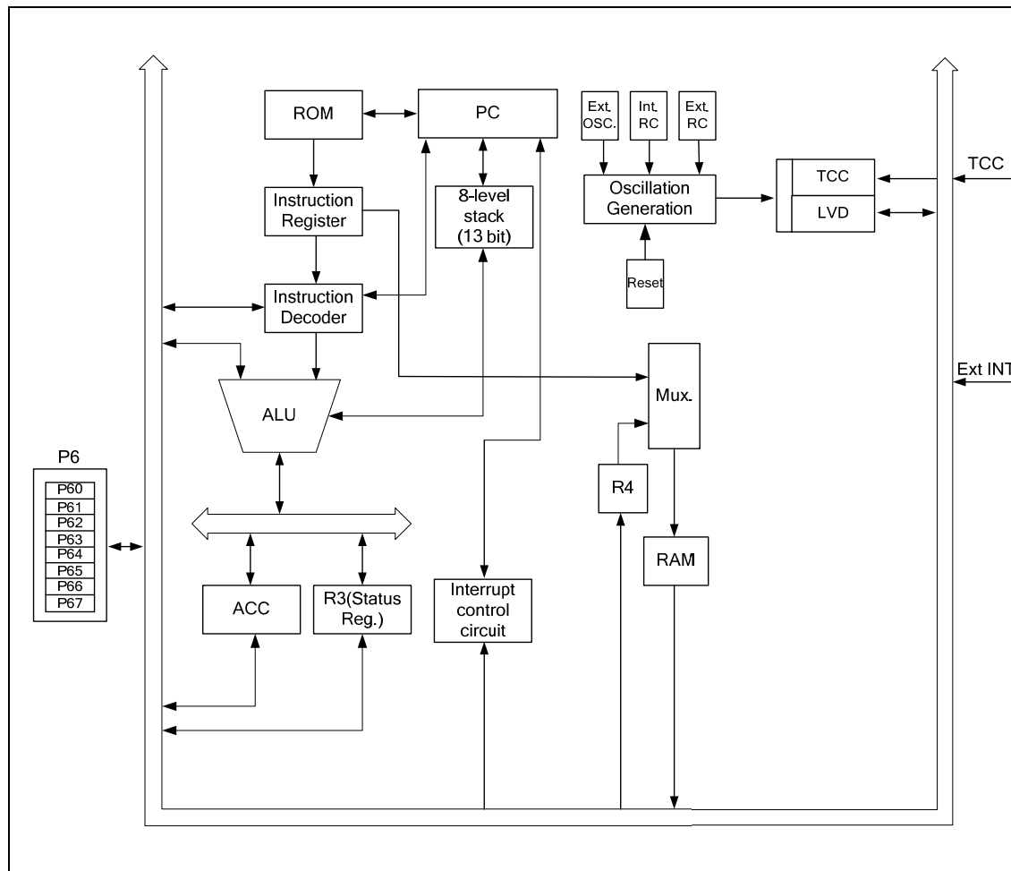
Figure 5-1 EM78P131A Functional Block Diagram
