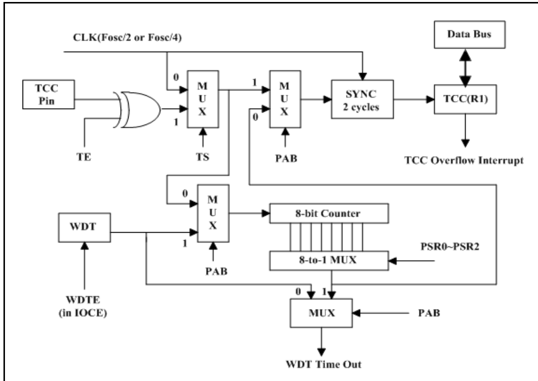
Figure 5-4 TCC and WDT Block Diagram
