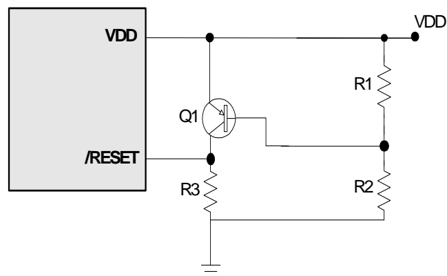
* Figure 5-16 Residue Voltage Protection Circuit 2
