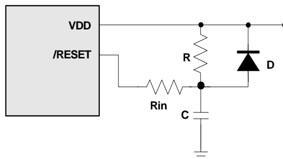
Fig 5-14 External Power-up Reset Circuit
