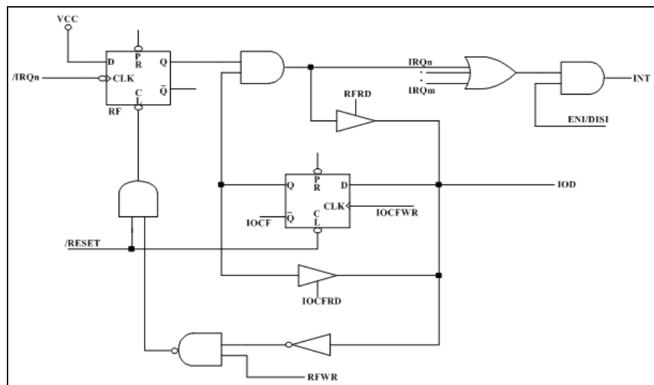
Figure 5-10 Interrupt Input Circuit
