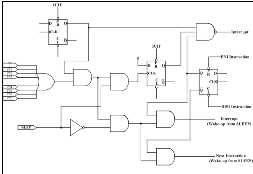
Fig. 5-8 Block Diagram of I/O Port 6 with input change interrupt/wake-up
