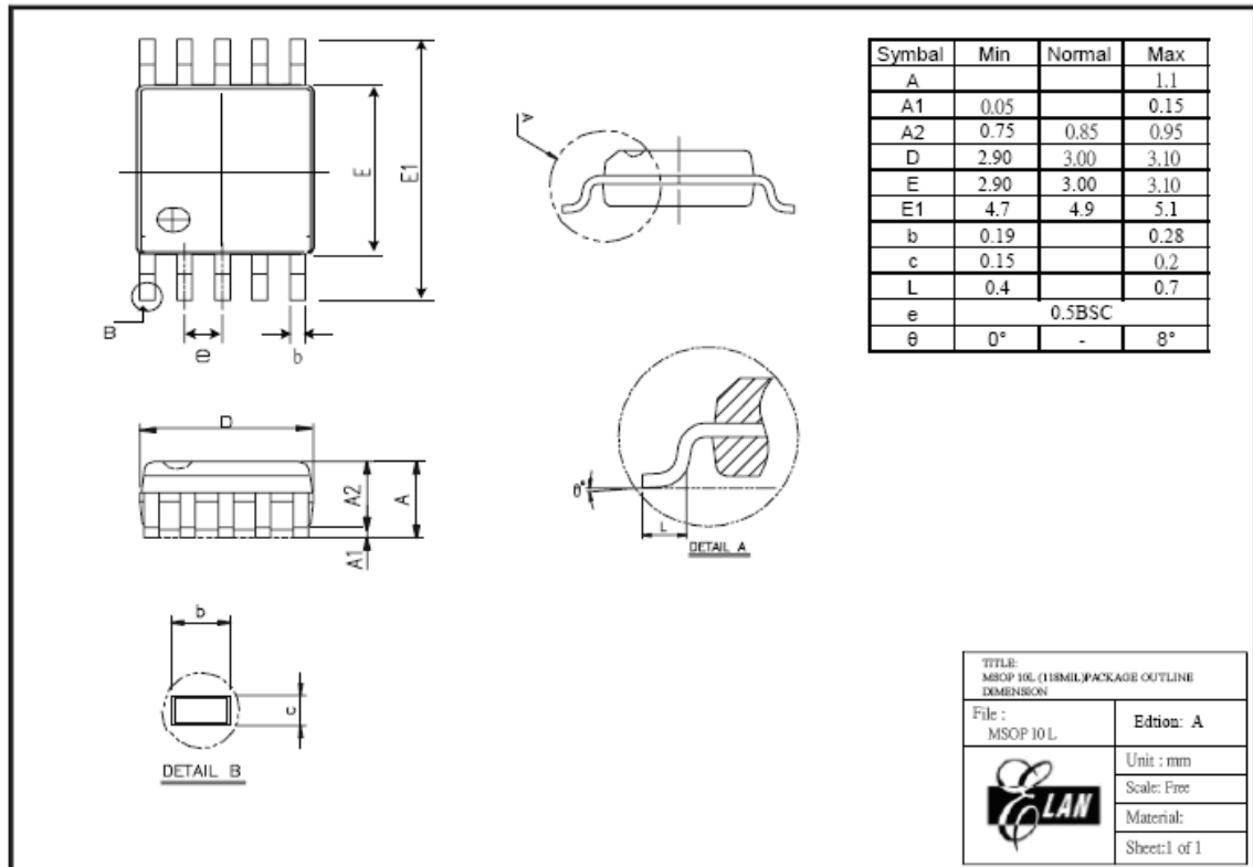
FigureB EM78P131A 10-Lead MSOP Package Type
