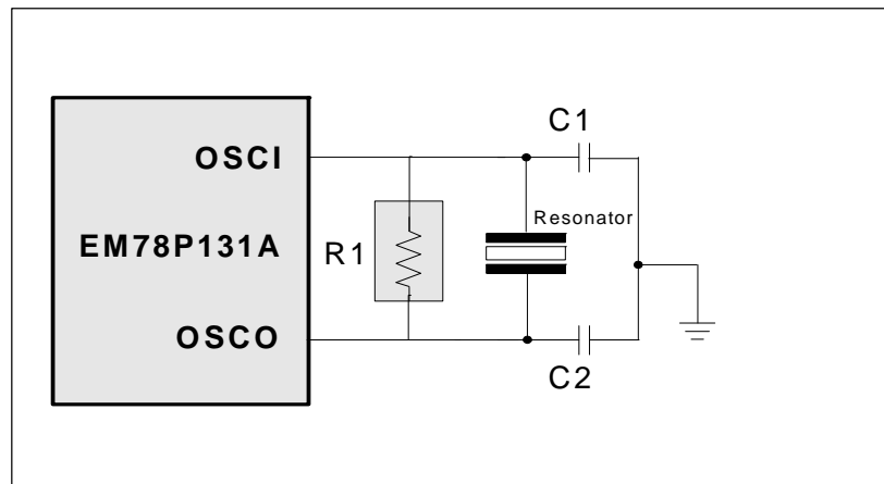
Fig. 5-12-1 Circuit for Crystal/Resonator
