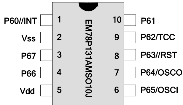
Figure 3-1 EM78P131AMS010J
