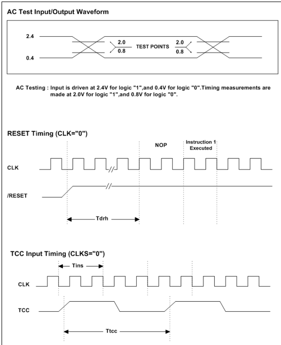
Figure 5-17 EM78P131A Timing Diagrams
