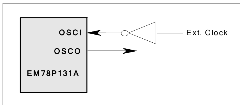
Fig. 5-11 Circuit for External Clock Input
