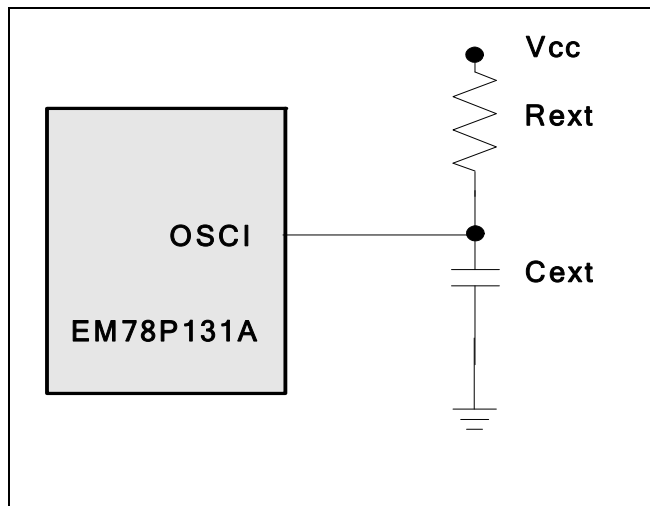
Figure 5-13 External RC Oscillator Mode Circuit
