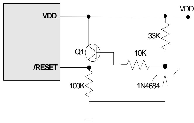
* Figure 5-15 Residue Voltage Protection Circuit 1
