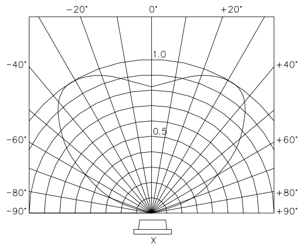
Radiation Diagram
