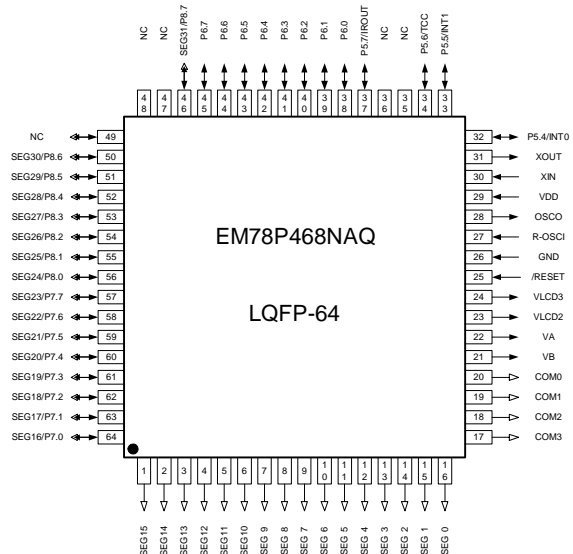
Fig. 3-2 64-pin LQFP
