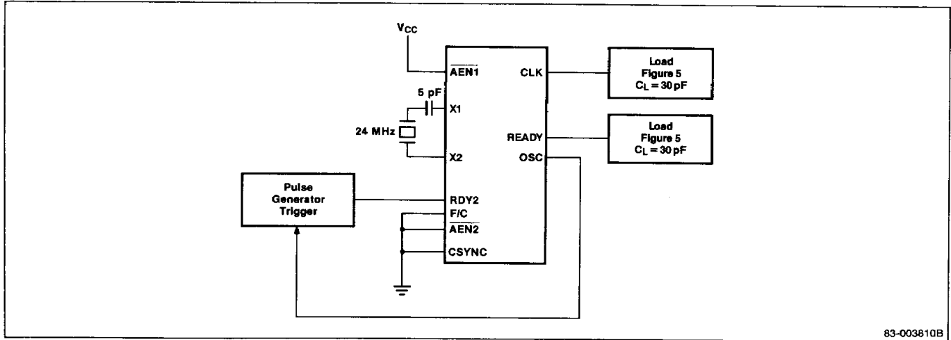
Figure 4. Ready to CLK Output
