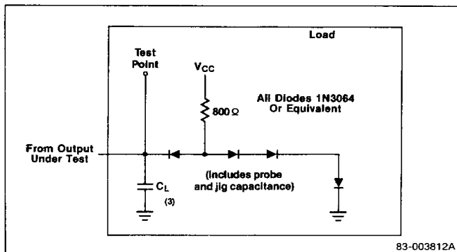
Figure 5. AC Load
