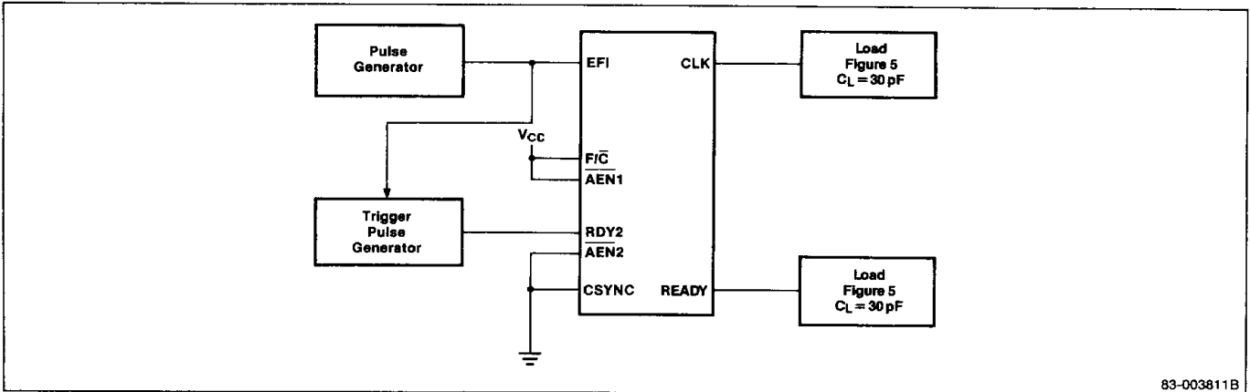
Figure 4. Ready to CLK Output
