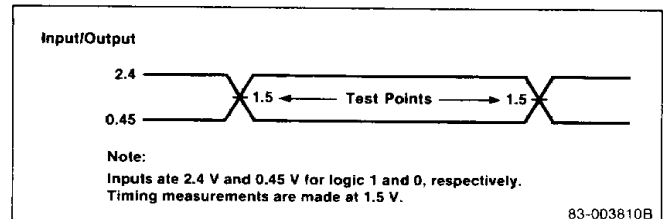
Figure 6. Timing Measurement Points
