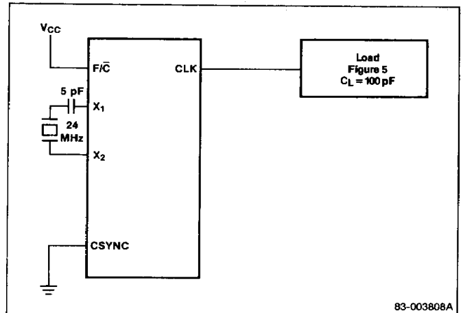
Figure 1. Clock High and Low Time
