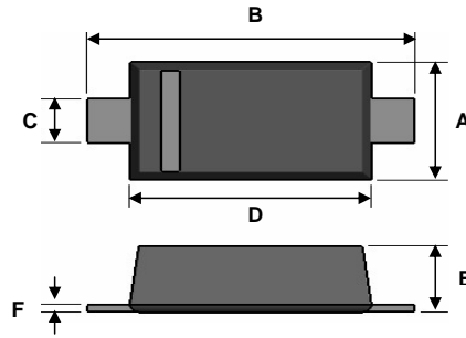
SOD-523F
