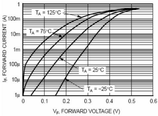
Figure 1. Forward Characteristics
