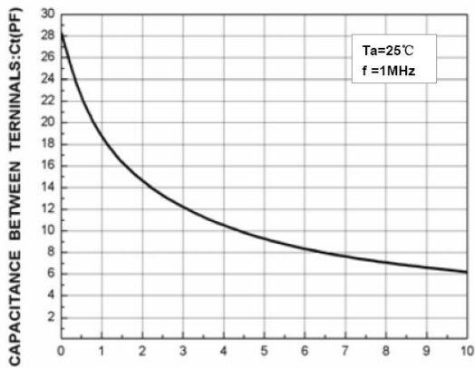
Figure3.Total Capacitance
