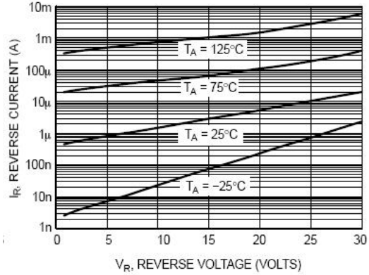
Figure 2. Reverse Characteristics
