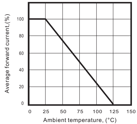
Fig.4 - Derating curve (Mounting on glass epoxy PCBs)
