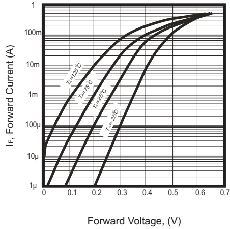
Fig.1 Forward Characteristics
