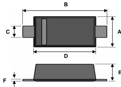
SOD-523F
