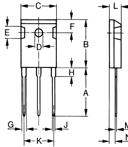
Dimensions TO-247AD
