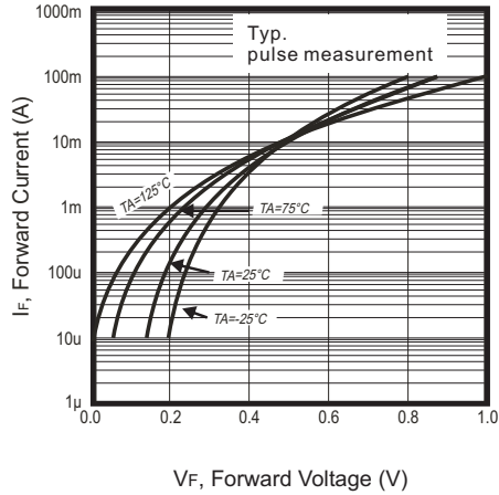
Fig. 1 - Forward Characteristics
