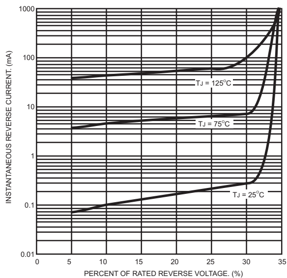
FIG.2- REVERSE CHARACTERISTICS
