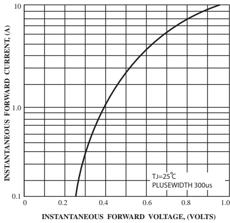
FIG3-TYPICAL FORWARD CHARACTERISTICS
