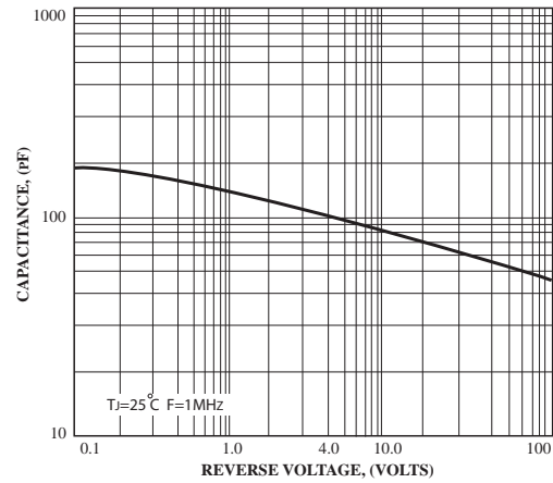
FIG4-TYPICAL JUNCTION CAPACITANCE
