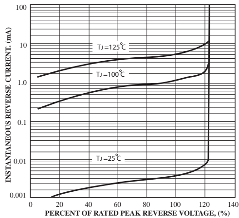
FIG5-TYPICAL REVERSE CHARACTERISTICS
