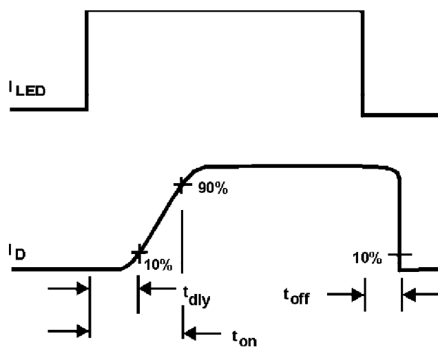
Figure 8. Delay Time Definitions
