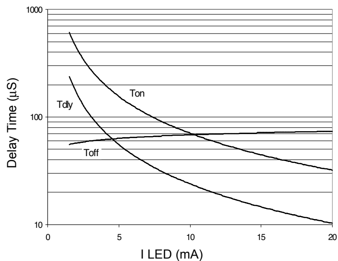
Figure 7. Typical Delay Times
