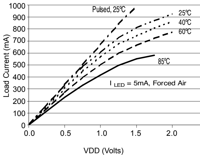
Figure 3. Typical On Characteristics
