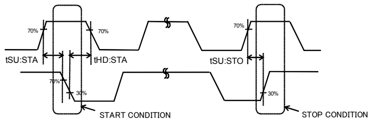
Fig.2-(b) Start-stop bit timing
