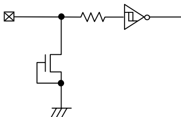
Fig.50 Input pin circuit diagram
