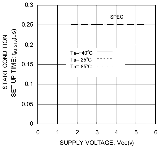
Fig.18 Start Condition Setup Time t_{SU:STA}
