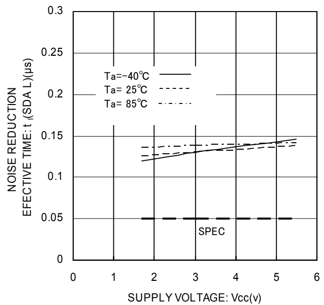
Fig. 31 Noise Spike Width t_i(SDA L)
