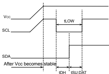
Fig.53 When SCL= 'H' and SDA= 'L'
