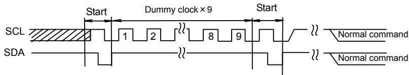
Fig.41-(b) The case of START + dummy clock × 9 +START+ command input
