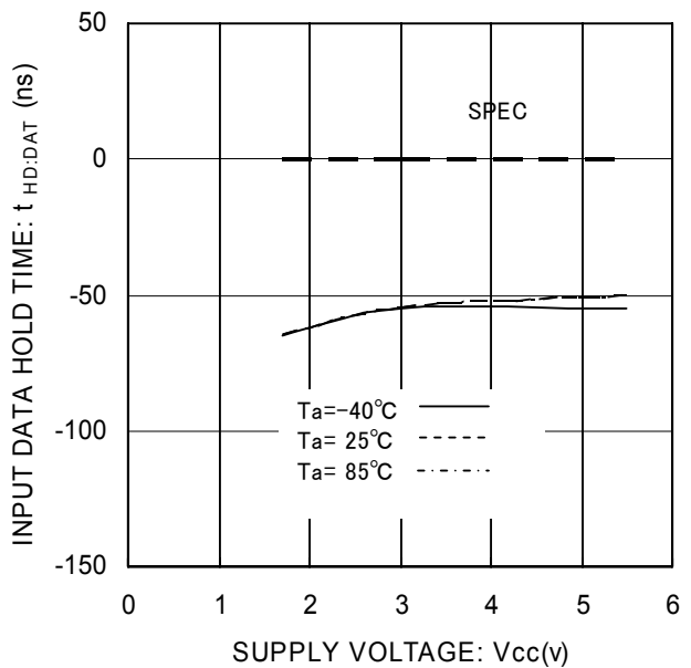
Fig.19 Input Data Hold Time t_{HD:DAT(HIGH)}
