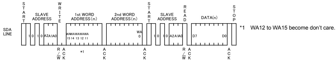
Fig.38 Random read cycle
