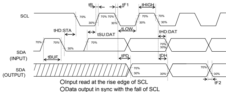
Fig.2-(a) Sync data input / output timing
