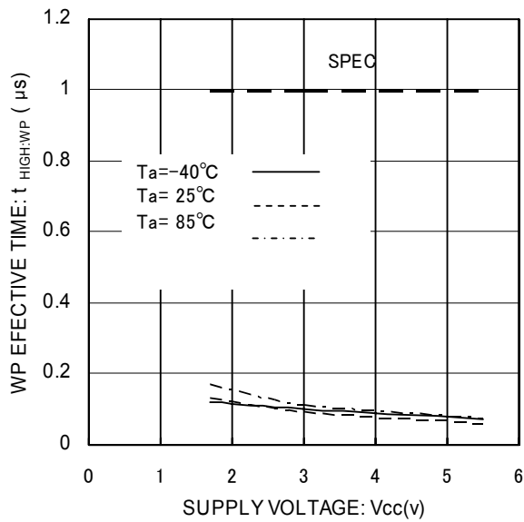
Fig. 34 WP High Time t_{HIGH:WP}
