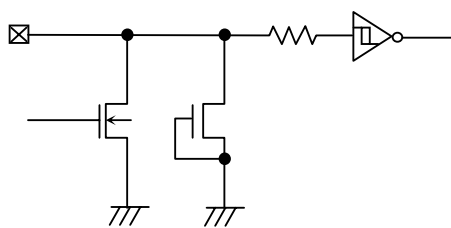
Fig.51 Input / output pin circuit diagram
