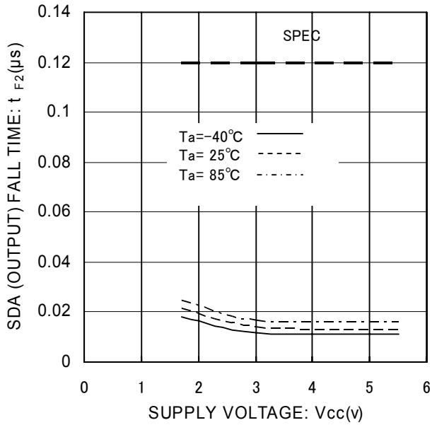
Fig.16 SDA (OUTPUT) Fall Time t_{F2}
