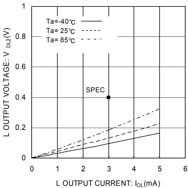
Fig. 6 'L' output voltage V_{OL1}(V_{CC}=2.5V)
