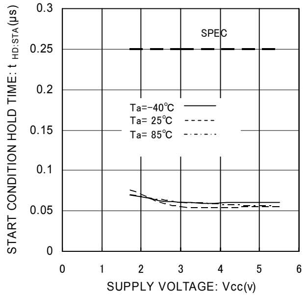
Fig.17 Start Condition Hold Time t_{HD:STA}
