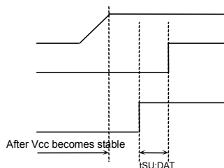
Fig.54 When SCL='L' and SDA='L'
