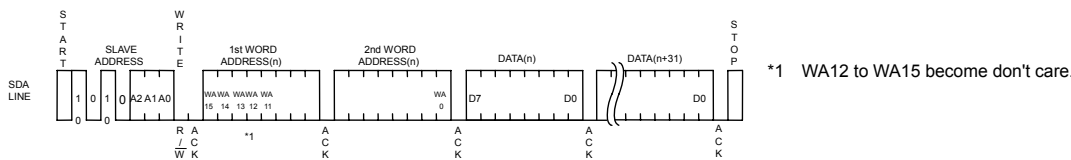
Fig.37 Page write cycle
