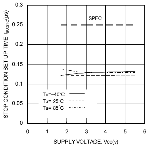
Fig.25 Stop Condition Setup Time t_{SU:STO}
