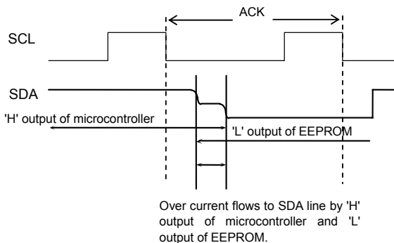
Fig.47 Input / output collision timing
