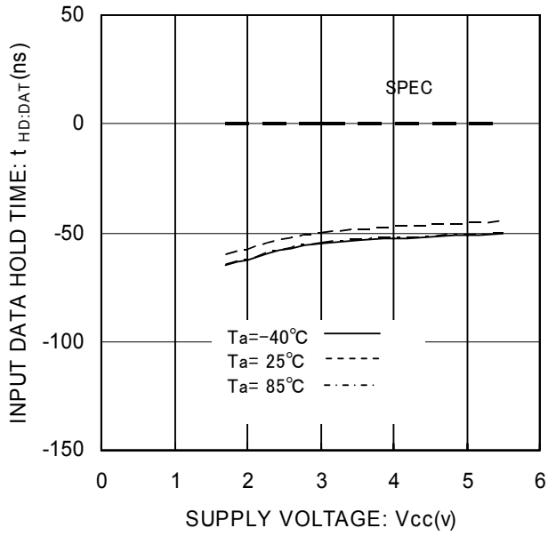
Fig.20 Input Data Hold Time t_{HD:DAT}(LOW)
