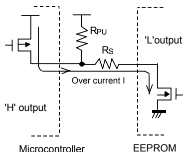
Fig.49 I/O circuit diagram
