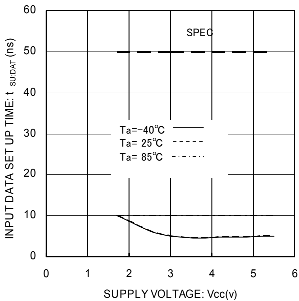
Fig.22 Input Data Setup Time t_{SU:DAT}(LOW)
