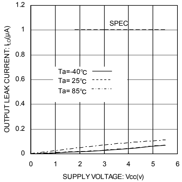
Fig.9 Output leak current I_{LO} (SDA)
