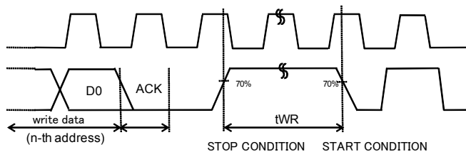
Fig.2-(c) Write cycle timing
