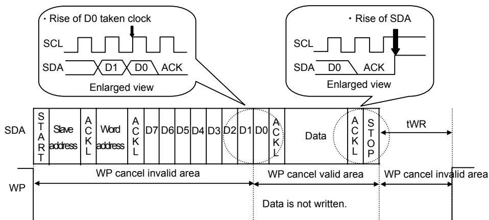
Fig.43 WP valid timing
