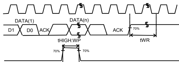
Fig.2-(e) WP timing at write cancel
