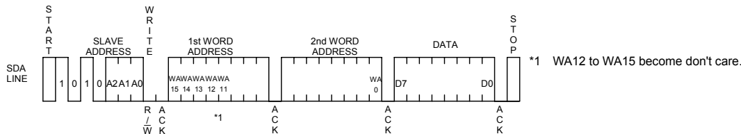
Fig.36 Byte write cycle
