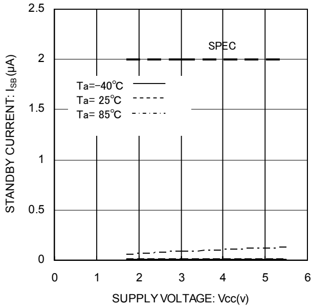
Fig.12 Standby operation I_{SB}
