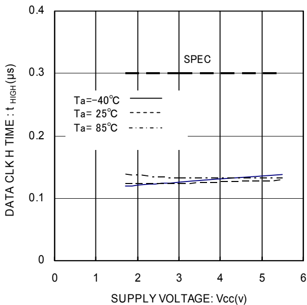
Fig.14 Data Clock High Period t_{HIGH}
