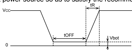
Fig.52 Rise waveform diagram
