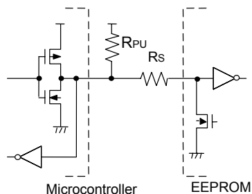
Fig.46 I/O circuit diagram
