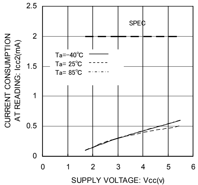
Fig.11 Current consumption at READ operation I_{CC2} ( f_{SCL}=1MHz )
