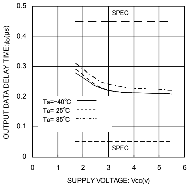
Fig.24 Output Data Delay Time t_{PD1}
