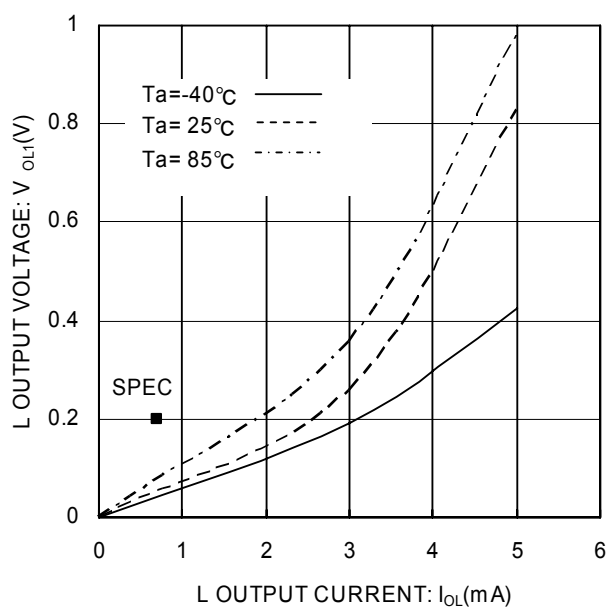
Fig.7 'L' output voltage V_{OL2}(V_{CC}=1.7V)
