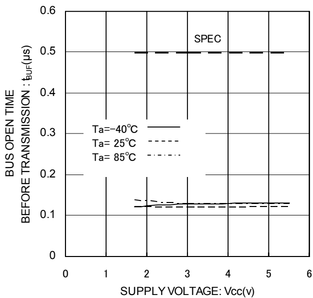
Fig.26 BUS Free Time t_{BUF}
