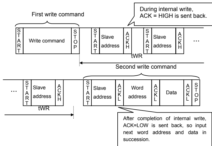
Fig.42 Case to continuously write by acknowledge polling
