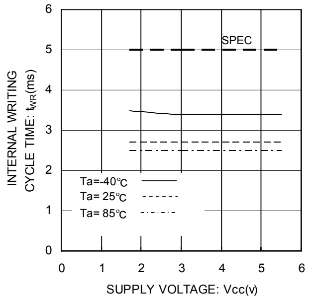
Fig.27 Write Cycle Time t_{WR}
