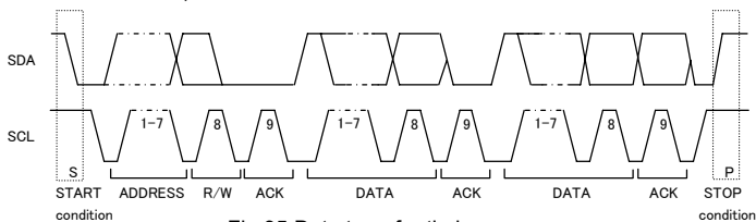
Fig.35 Data transfer timing
