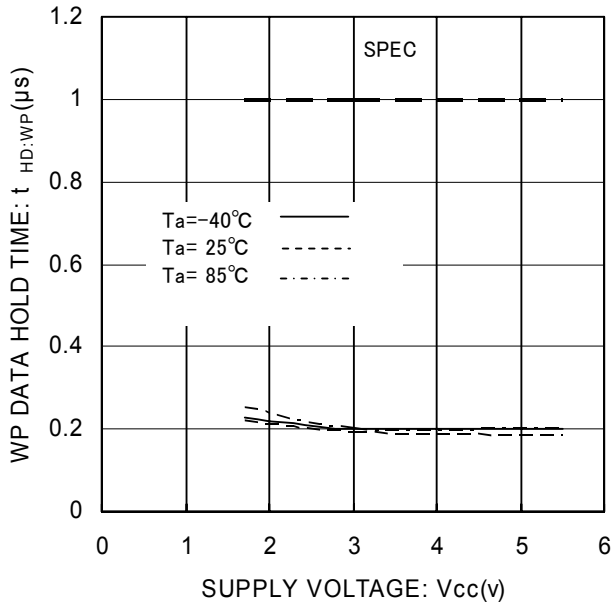
Fig. 32 WP Hold Time t_{HD:WP}
