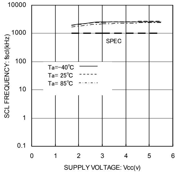
Fig.13 Clock Frequency f_{SCL}
