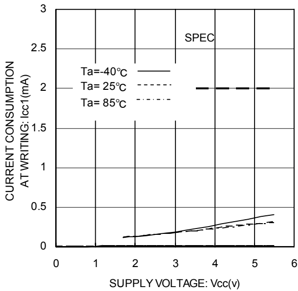
Fig.10 Current consumption at WRITE operation I_{CC1}
