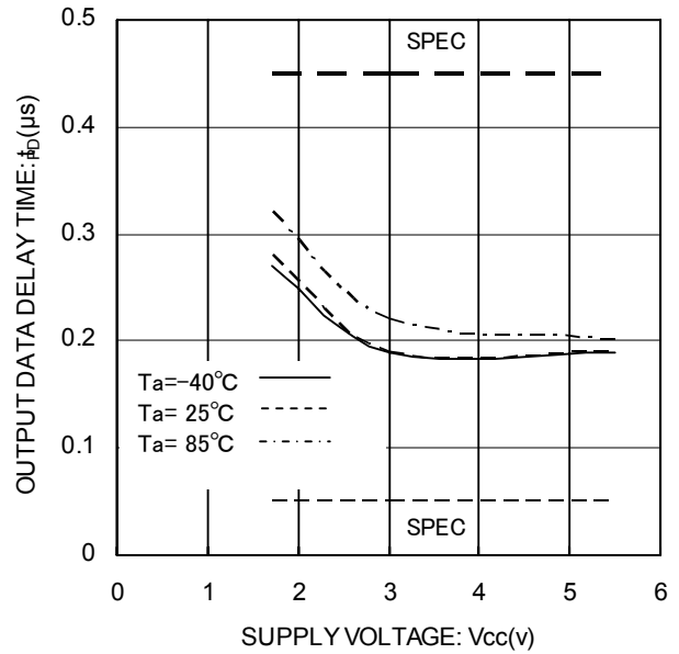
Fig.23 Output Data Delay Time t_{PD0}
