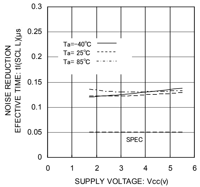
Fig. 29 Noise Spike Width t_i(SCL L)
