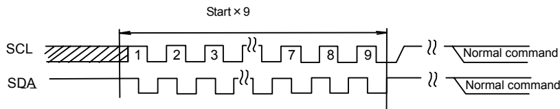
Fig.41-(c) START×9+ command input
