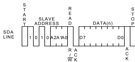
Fig.39 Current read cycle
