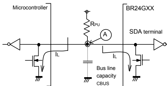
Fig.45 I/O circuit diagram
