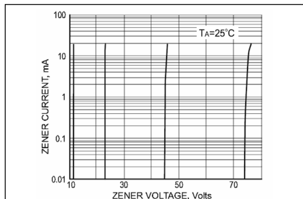
Fig.6 ZENER BREAKDOWN CHARACTERISTICS
