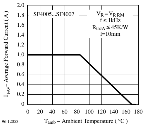
Figure 5. Max. Average Forward Current vs. Ambient Temperature
