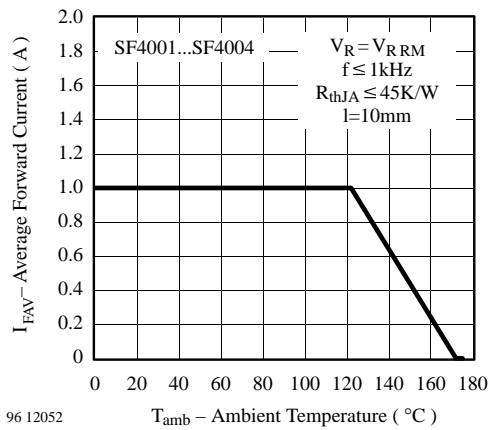
Figure 4. Max. Average Forward Current vs. Ambient Temperature
