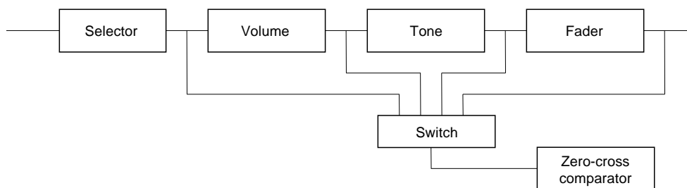
LC75410E, 75410W Zero-Cross Detection Circuit
