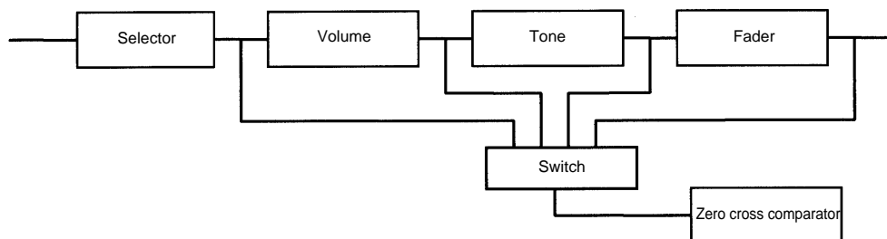
Zero Cross Detection Circuit
