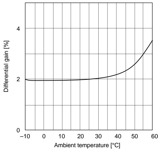
Differential gain vs. Ambient temperature
