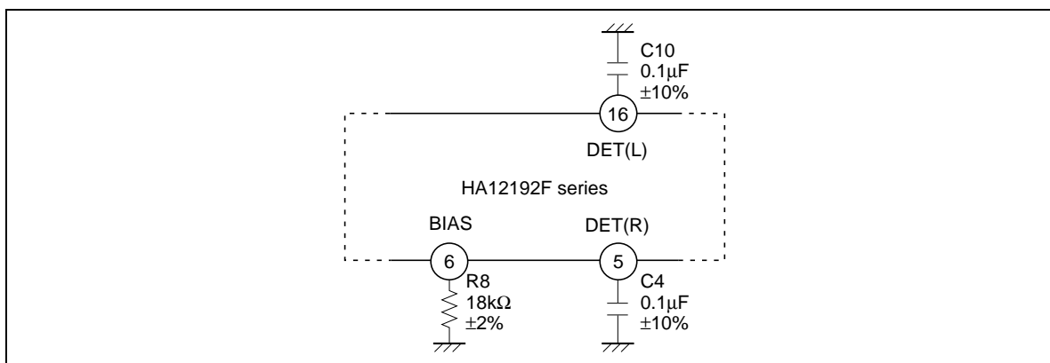
Figure 6 Tolerance of External Components
