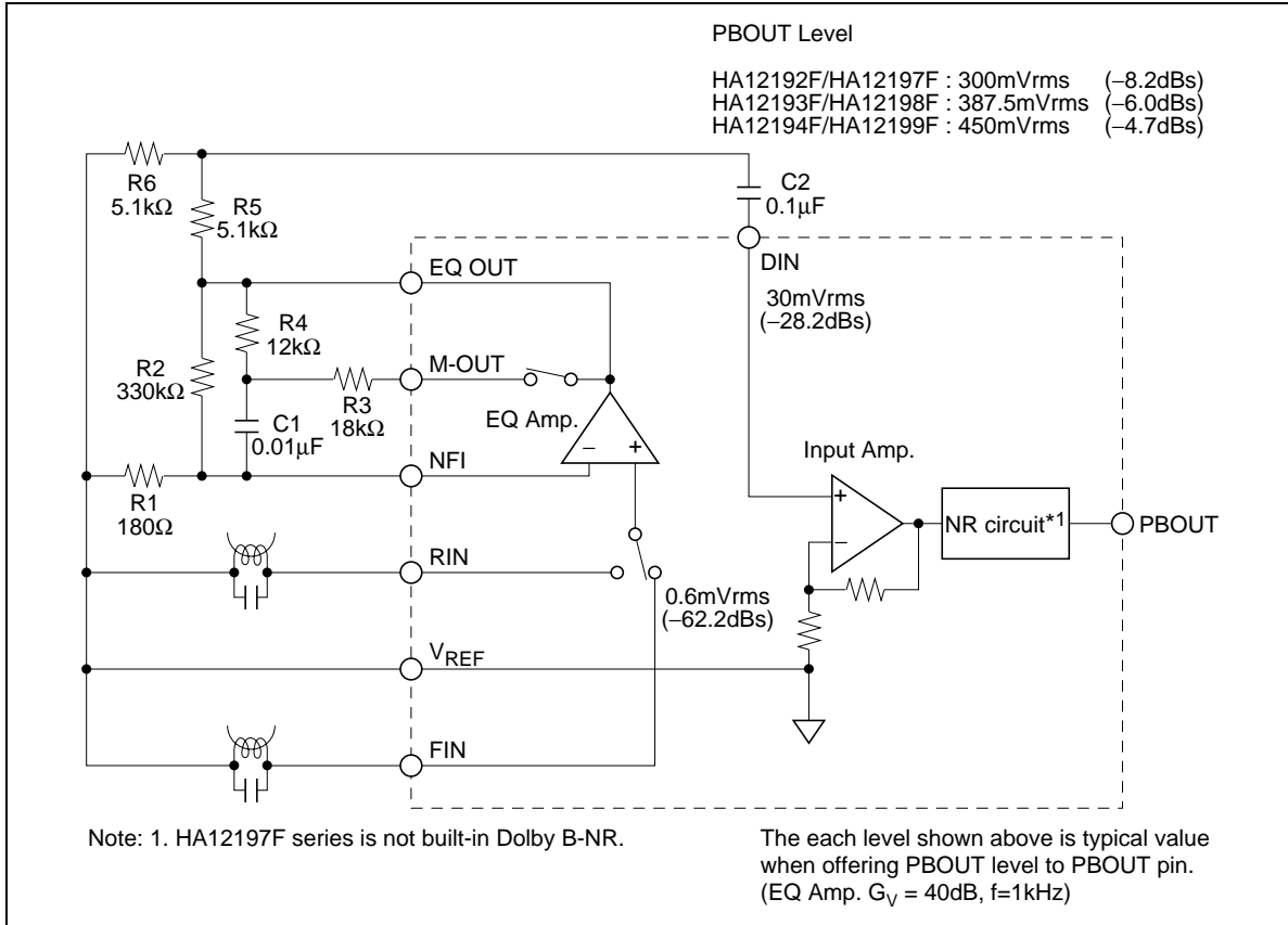
Figure 3 Input Block Diagram
