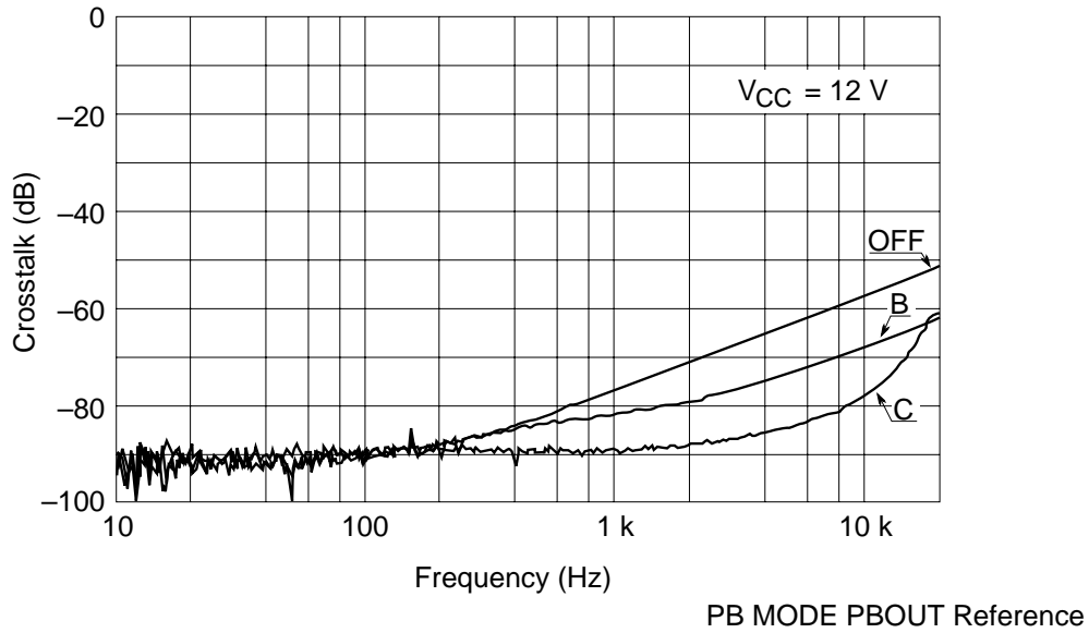
Crosstalk vs. Frequency (REC→PB)
