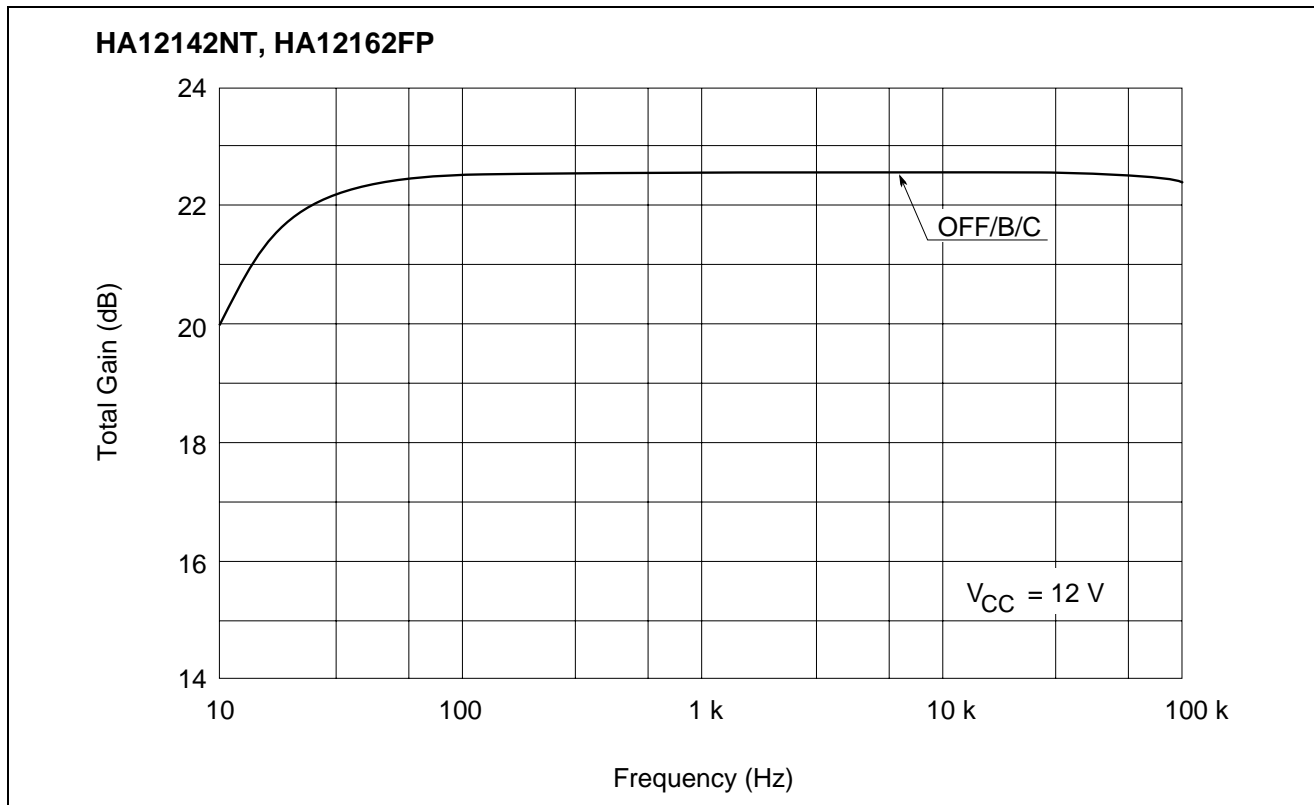
Total Gain vs. Frequency (REC MODE PBOUT)
