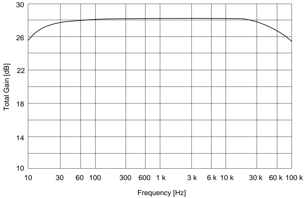
Total Gain vs. Frequency (PB MODE PBOU NR-OFF V_{cc} = 14 V)
