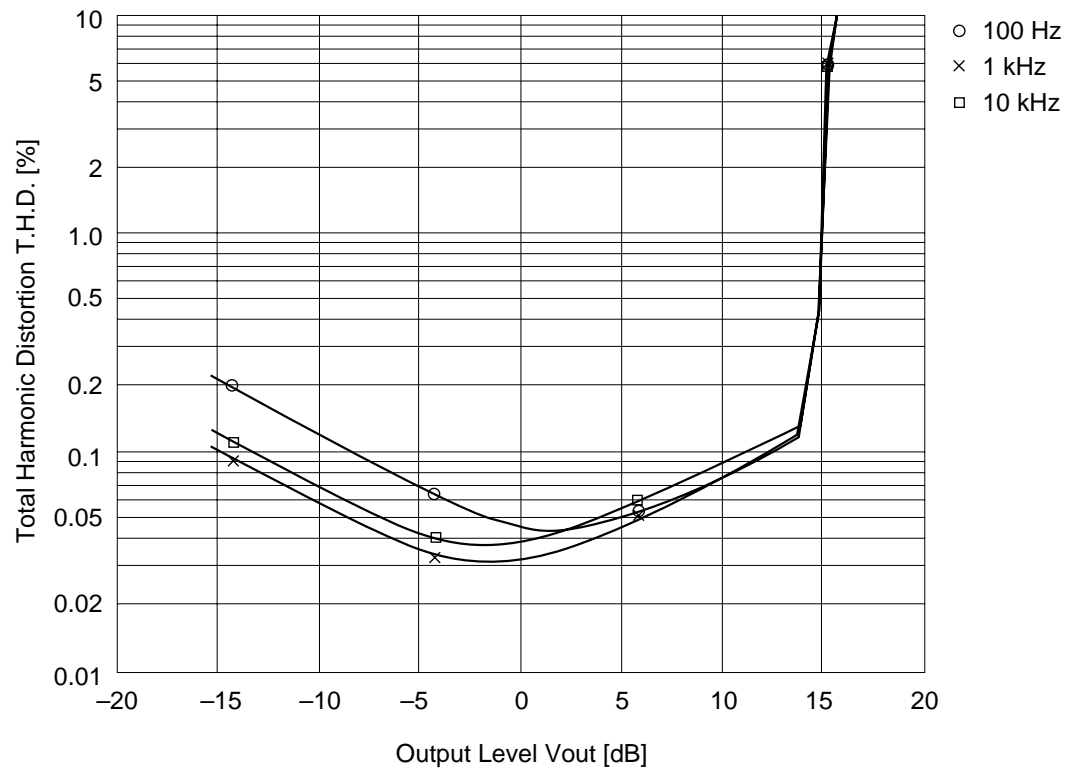
Total Harmonic Distortion vs. Output Level (REC MODE NR-OFF V_{cc} = 14 V)
