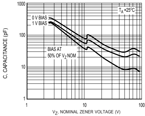
Figure 7 Typical Capacitance
