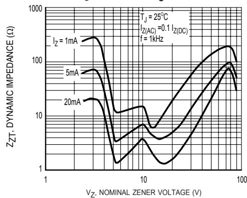
Figure 5 Effect of Zener Voltage on Zener Impedance
