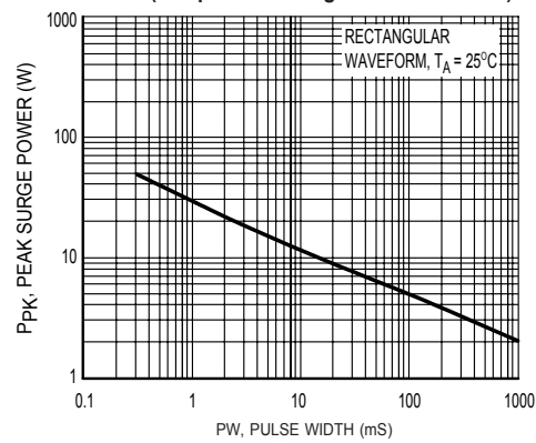
Figure 4 Maximum Nonrepetitive Surge Power
