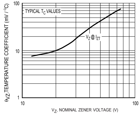
Figure 2 Temperature Coefficients (Temperature Range -55°C to +150°C)
