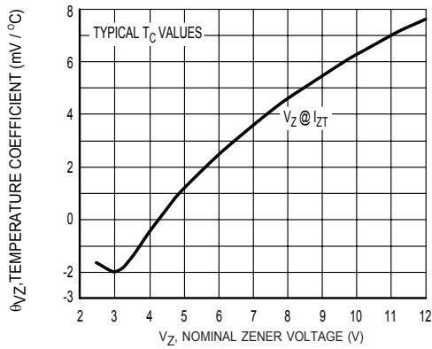
Figure 1 Temperature Coefficients (Temperature Range -55°C to +150°C)
