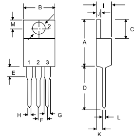
TO-220AB
