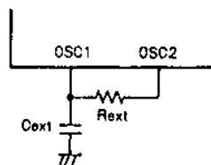
Fig. 3 2-Pin RC Oscillation Circuit
