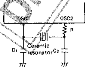
Fig. 2 Ceramic Resonator Oscillation Circuit
