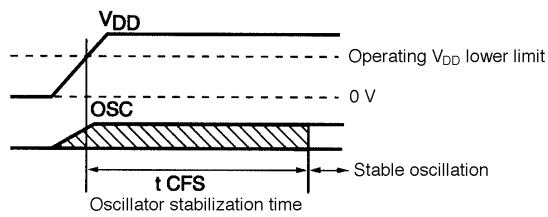
Figure 4 Oscillator Stabilization Time
