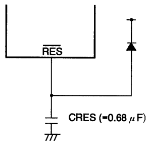
Figure 6 Reset Circuit
