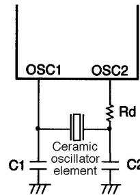
Figure 3 Ceramic Oscillator Circuit
