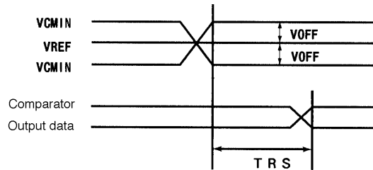
Figure 5 Comparator Response Speed TRS Timing
