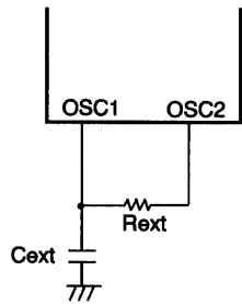
Figure 2 Two-Pin RC Oscillator Circuit
