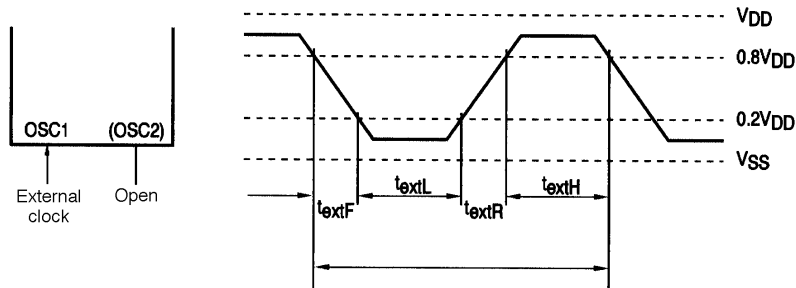
Figure 1 External Clock Input Waveform
