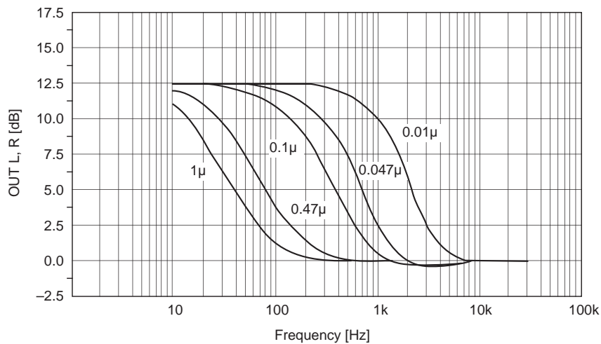
CH. vs. BASS-CONTROL (MAX)
