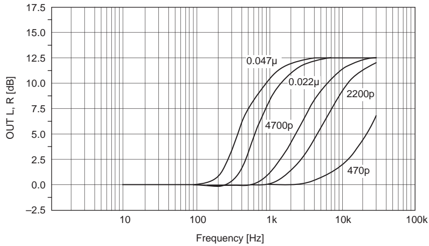
CH. vs. TREBLE-CONTROL (MAX)
