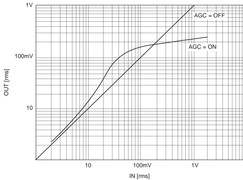
AGC characteristics
