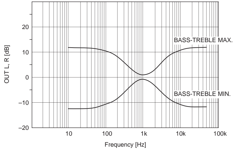
TONE characteristics
