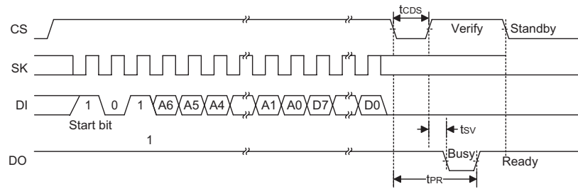
WRITE Timing
