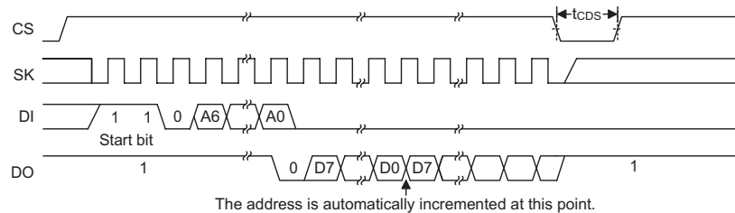
READ Timing
