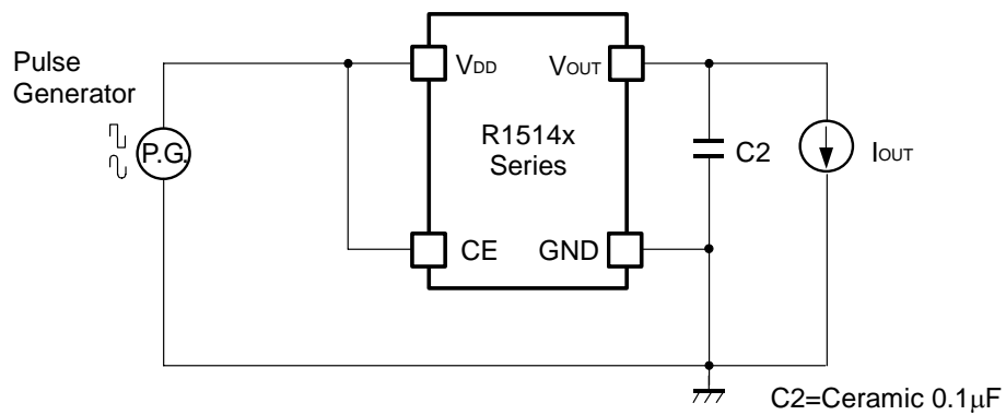
Test Circuit for Line Transient Response
