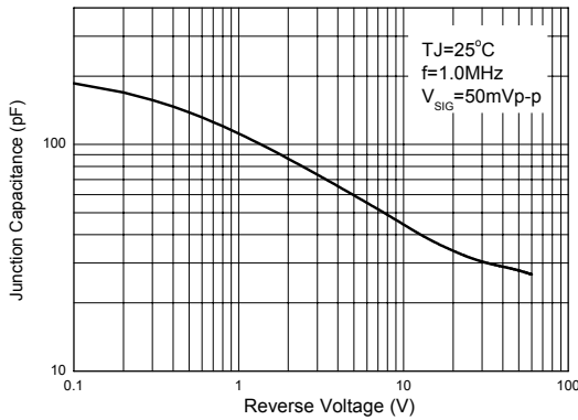
Figure 7. Typical Junction Capacitance
