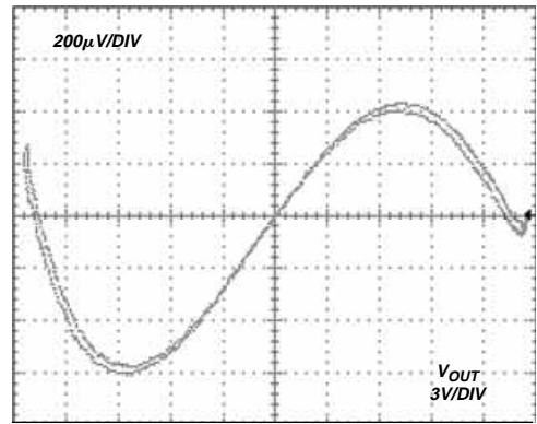
Figure 30. Gain Nonlinearity, V_S = \pm 15\text{ V} , G = +5 (7 ppm/DIV)
