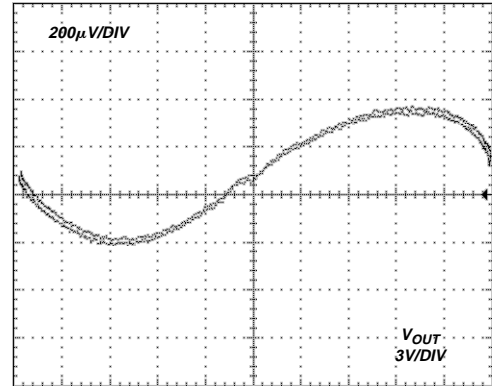
Figure 29. Gain Nonlinearity, V_S = \pm 15\text{ V} , G = 100 (7 ppm/DIV)
