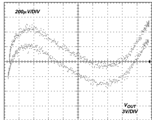
Figure 31. Gain Nonlinearity, V_S = \pm 15\text{ V} , G = +100 (7 ppm/DIV)
