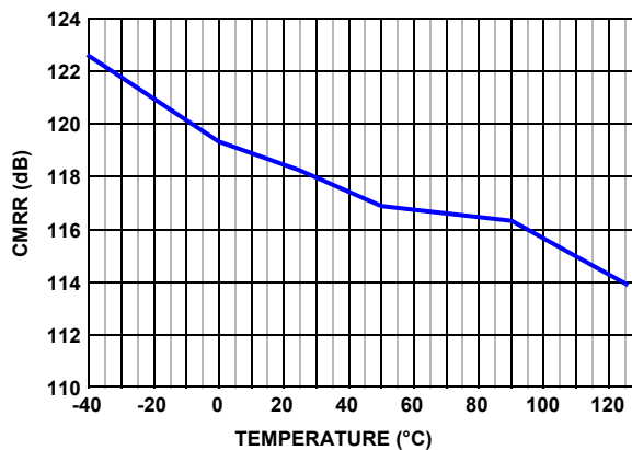
FIGURE 16. ISL28118 CMRR vs TEMPERATURE, V_S = \pm 5V
