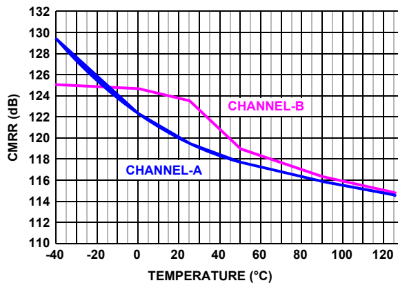
FIGURE 18. ISL28218 CMRR vs TEMPERATURE, V_S = \pm 5V
