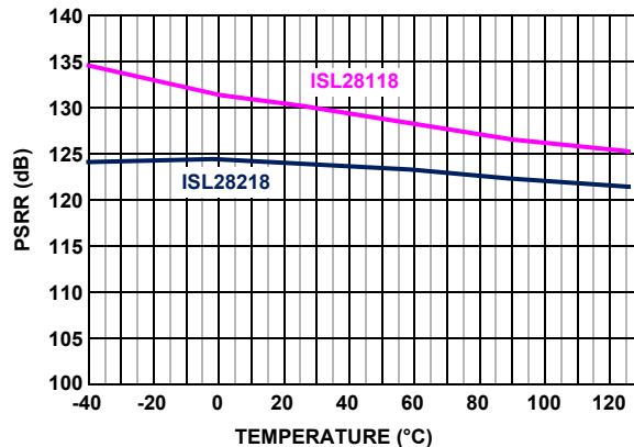
FIGURE 20. PSRR vs TEMPERATURE, V_S = \pm 15V
