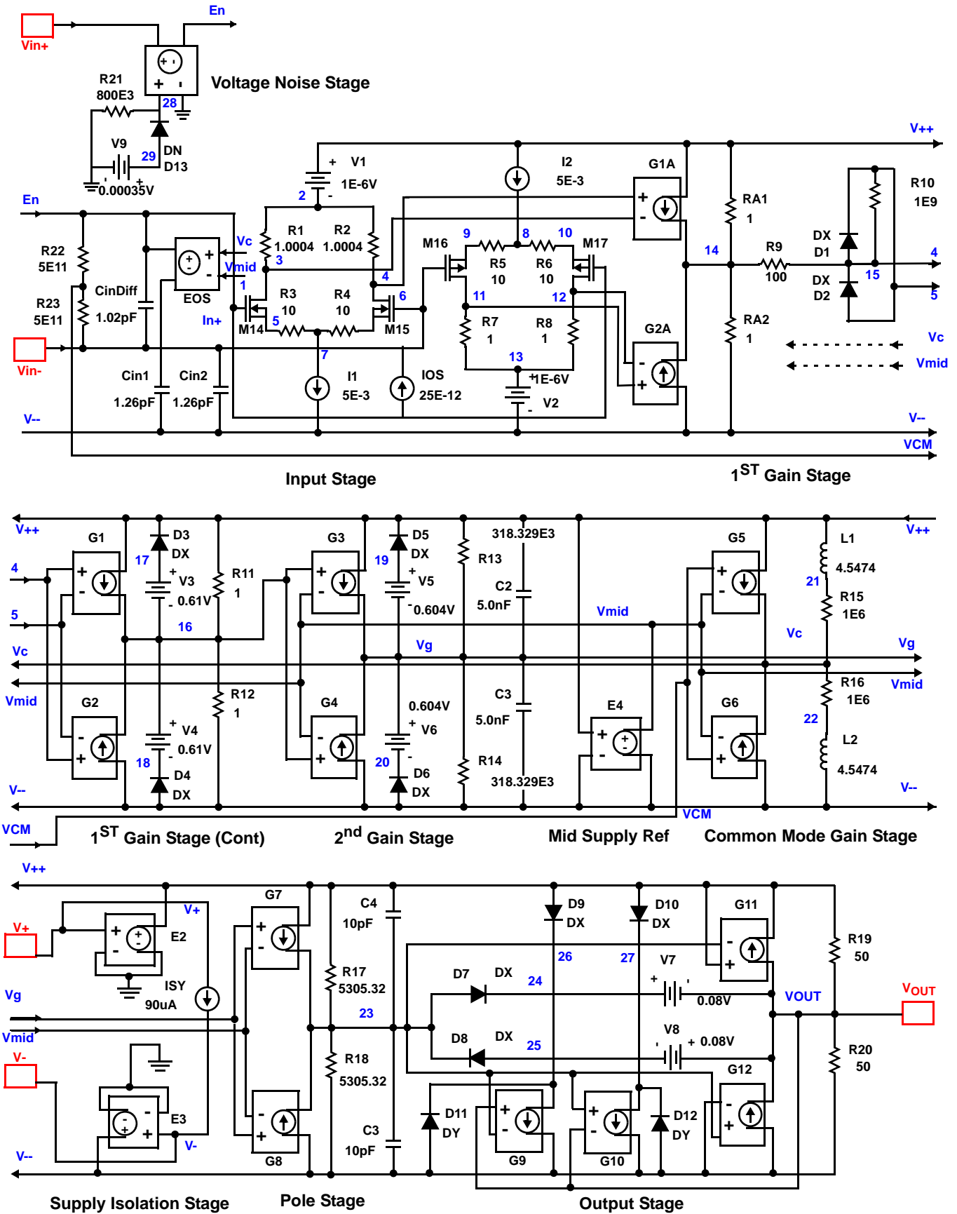
FIGURE 20. SPICE SCHEMATIC
