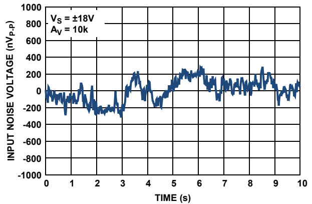
FIGURE 16. 0.1Hz TO 10Hz V_{P,P} NOISE VOLTAGE, V_S = \pm 18V
