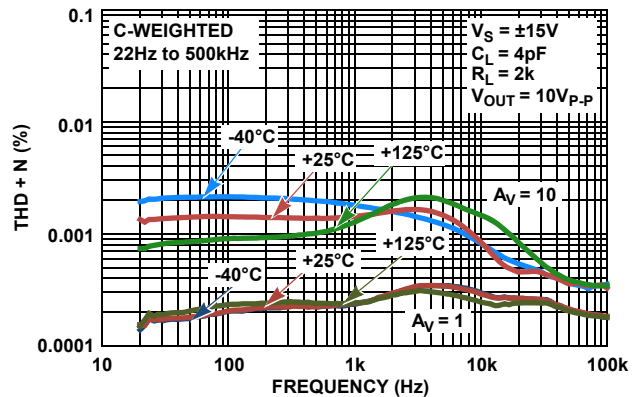
FIGURE 18. THD+N vs FREQUENCY vs TEMPERATURE, V_{OUT} = 10V_{P,P} , R_L = 2K\Omega
