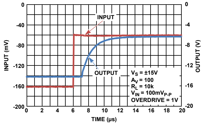
FIGURE 30. NEGATIVE OUTPUT OVERLOAD RECOVERY TIME
