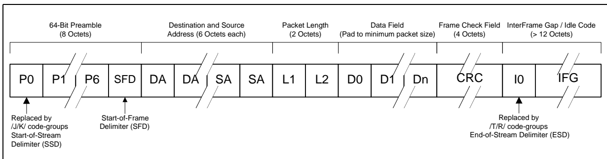
Figure 14. 100BASE-TX Data Path
