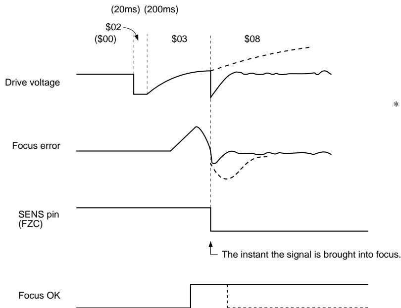
Fig. 4. Focus ON timing chart
