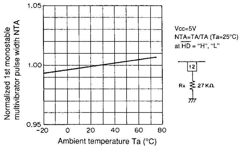
Normalized 1st monostable multivibrator pulse width NTA vs. Ambient temperature Ta
