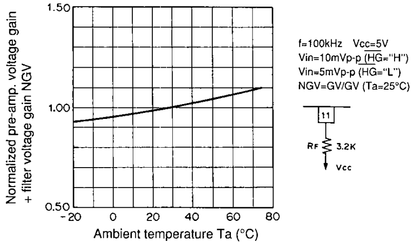
Normalized pre-amp. voltage gain + filter voltage gain NGV vs. Ambient temperature Ta
