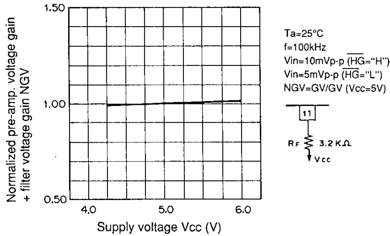
Normalized pre-amp. voltage gain + filter voltage gain NGV vs. Supply voltage Vcc
