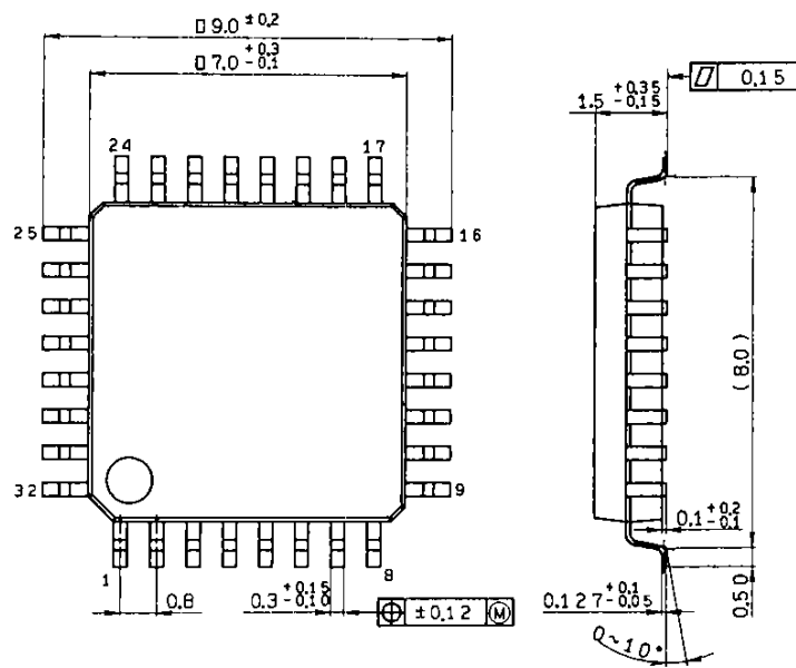
QFP-32P-L01
