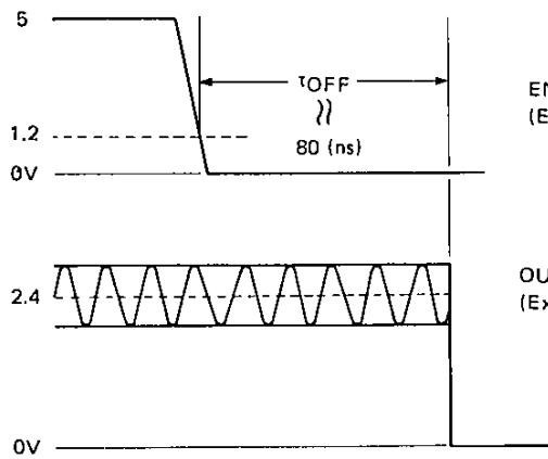
(a) Switching time t_{OFF}
