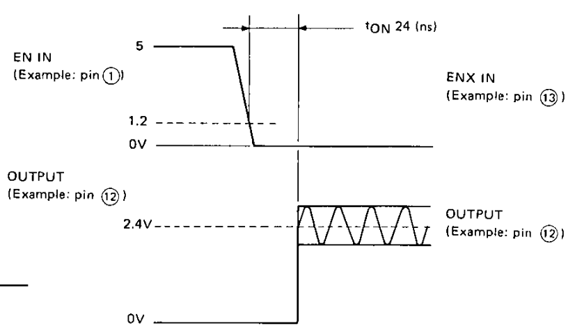
(b) Switching time t_{ON}
