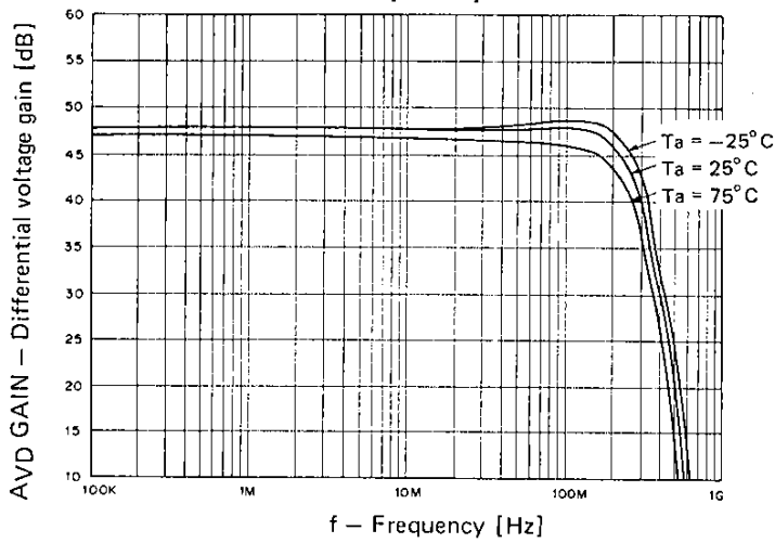
Temperature dependability of frequency characteristics
