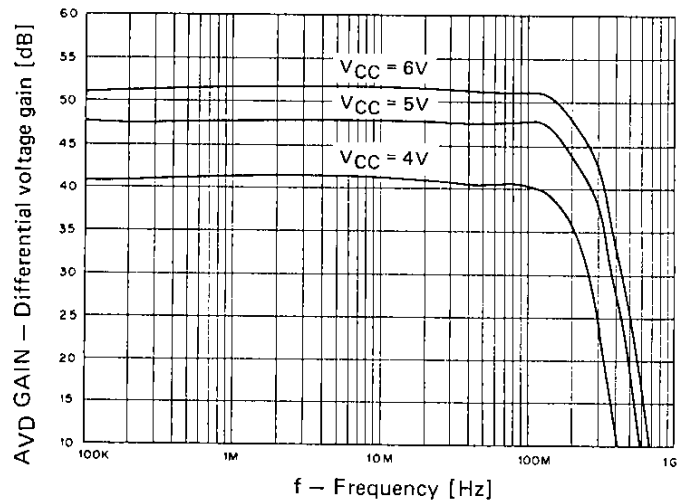
Frequency characteristics
