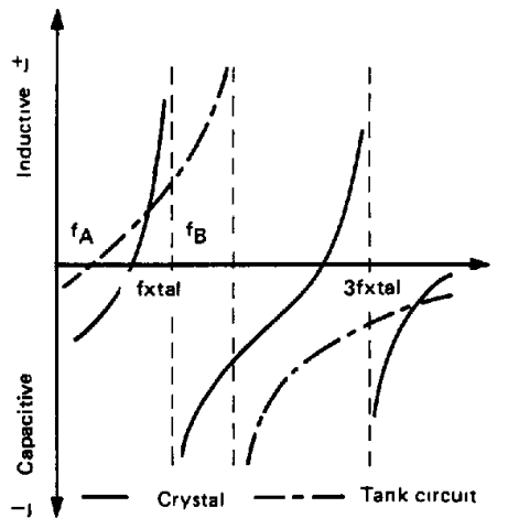
Reactance characteristics
