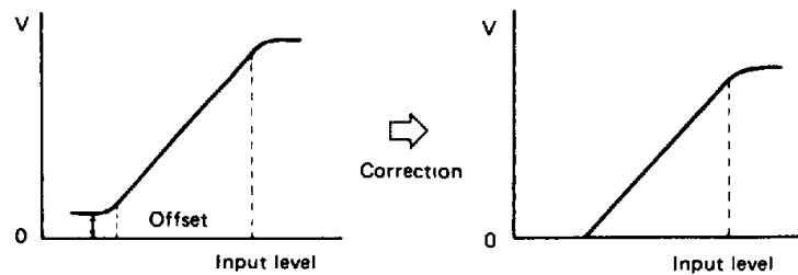
Offset correction of RSSI output voltage
