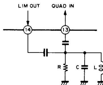
RLC phase shifter
