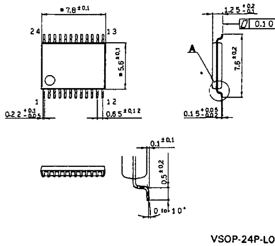
CXA1003BN 24 pin VSOP (Plastic)
