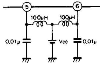
Power supply decoupling
