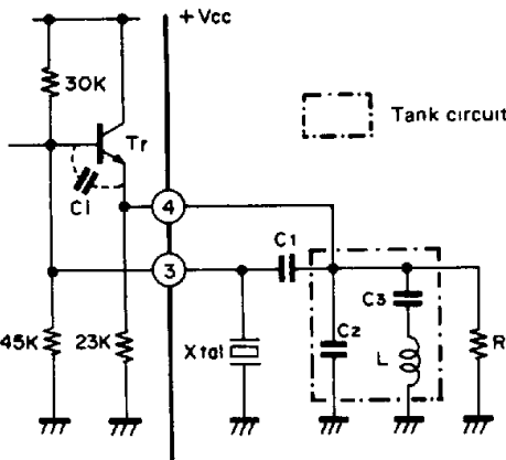
Colpitts type crystal oscillation circuit
