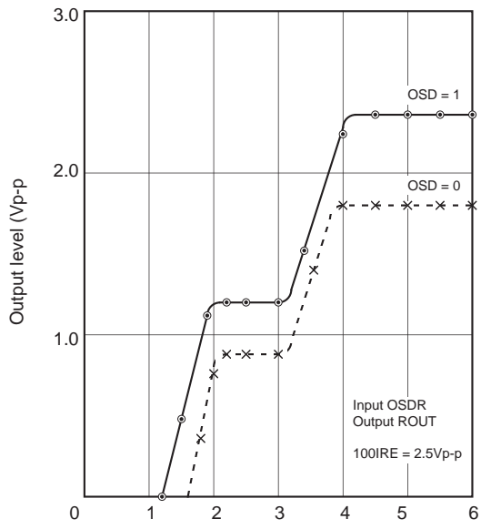
Fig 12. OSD RGB I/O characteristics
