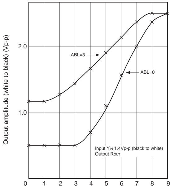
Fig 10. ABL characteristics (picture)
