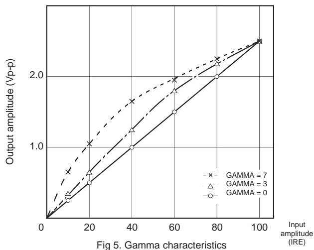
Fig 5. Gamma characteristics
