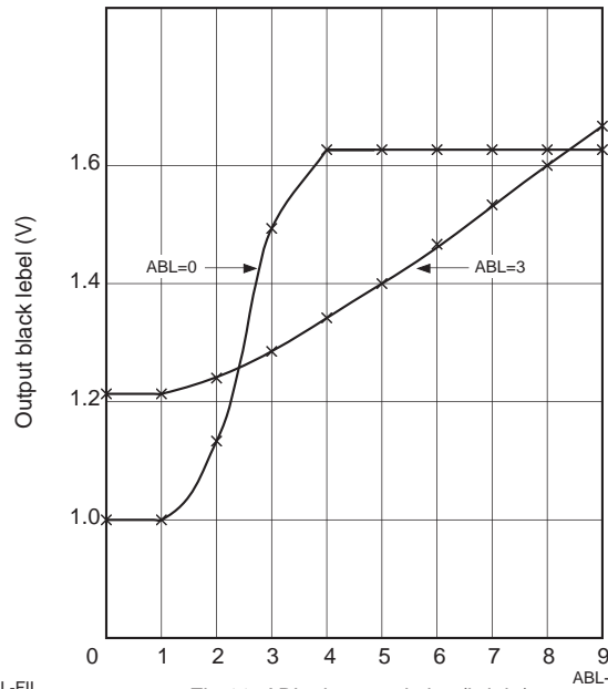
Fig 11. ABL characteristics (bright)
