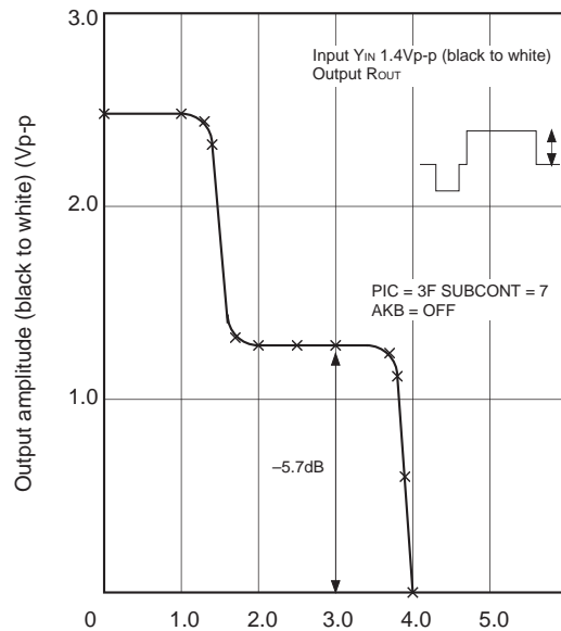
Fig 13. OSD-BLK voltage
