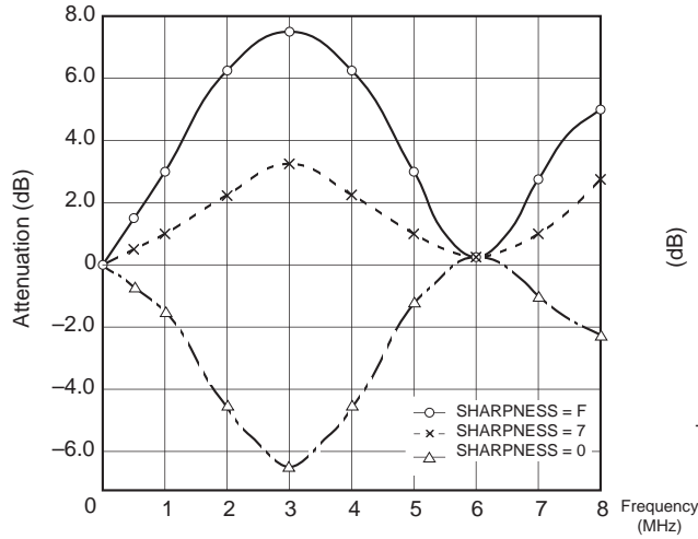
Fig 1. Sharpness characteristics
