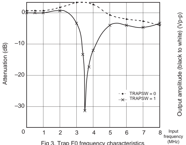
Fig 3. Trap F0 frequency characteristics
