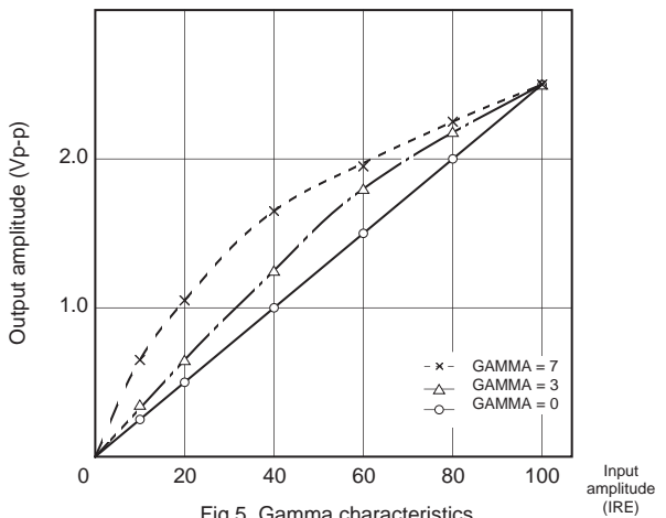
Fig 5. Gamma characteristics
