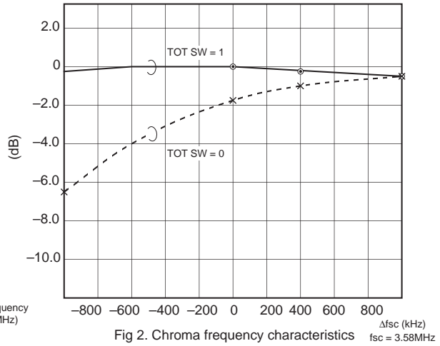
Fig 2. Chroma frequency characteristics
