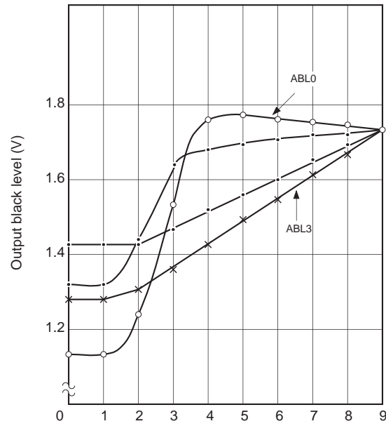
Fig 11. ABL characteristics (bright)
