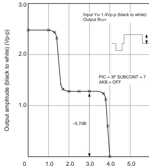
Fig 13. OSD-BLK voltage
