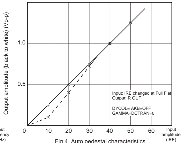
Fig 4. Auto pedestal characteristics
