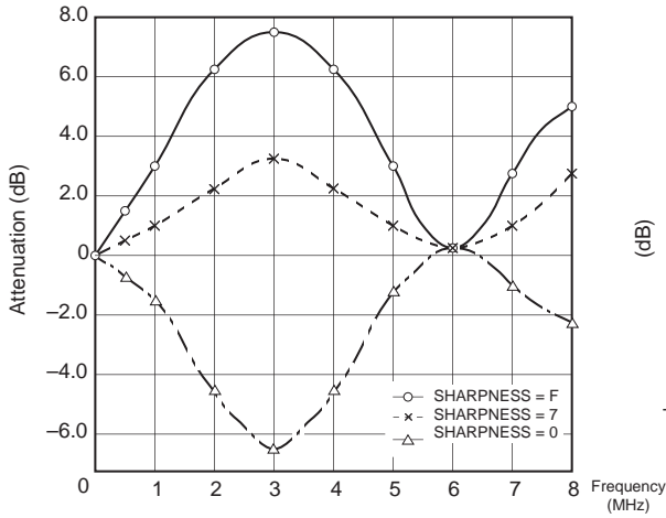
Fig 1. Sharpness characteristics
