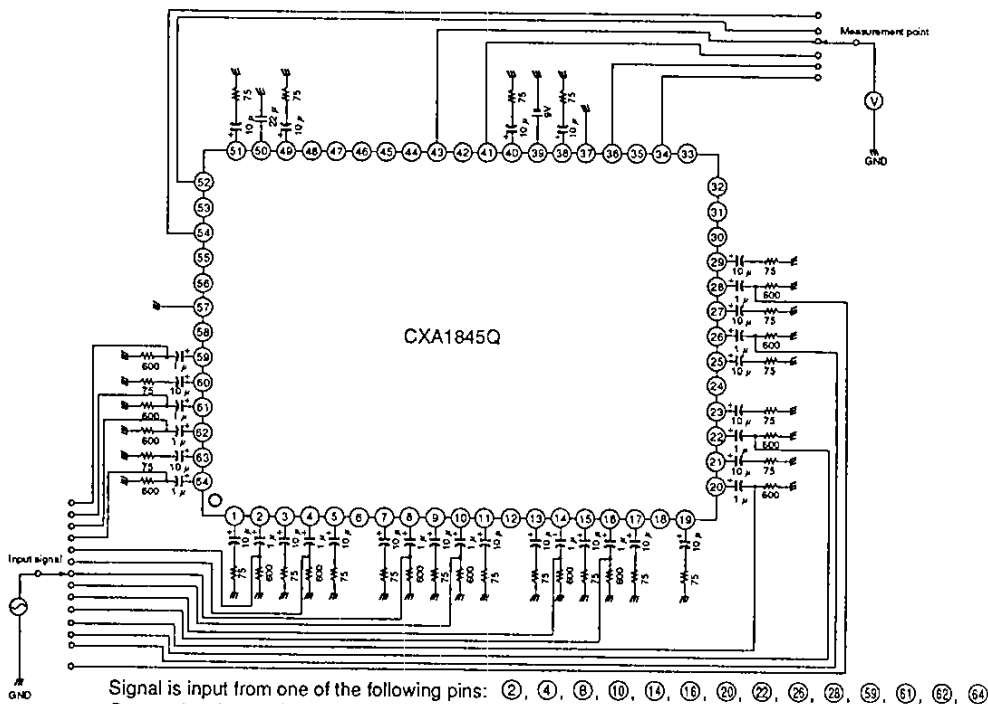
Fig. 4 Audio system (cross talk)
