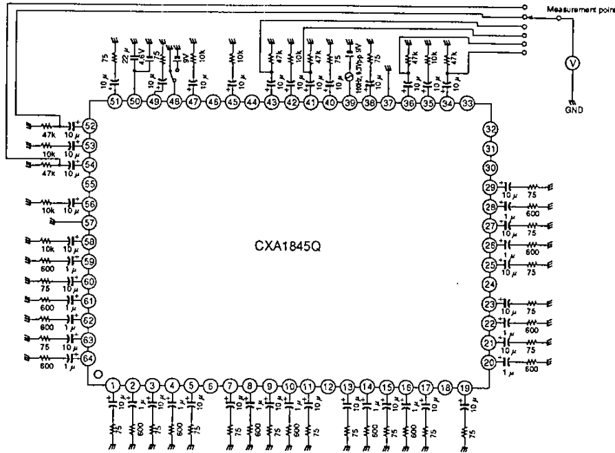
Fig. 5 Audio system (ripple rejection)
