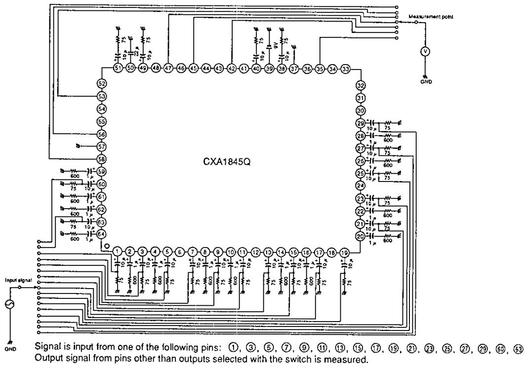
Fig. 2 Video system (cross talk)
