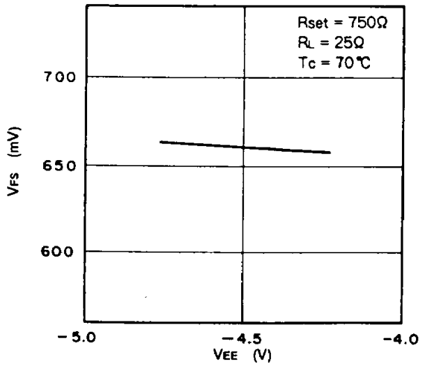
Full gray balance vs. Supply voltage
