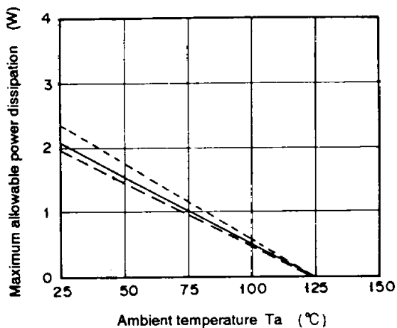
(b) Air Flow Rate 1.5m/sec
