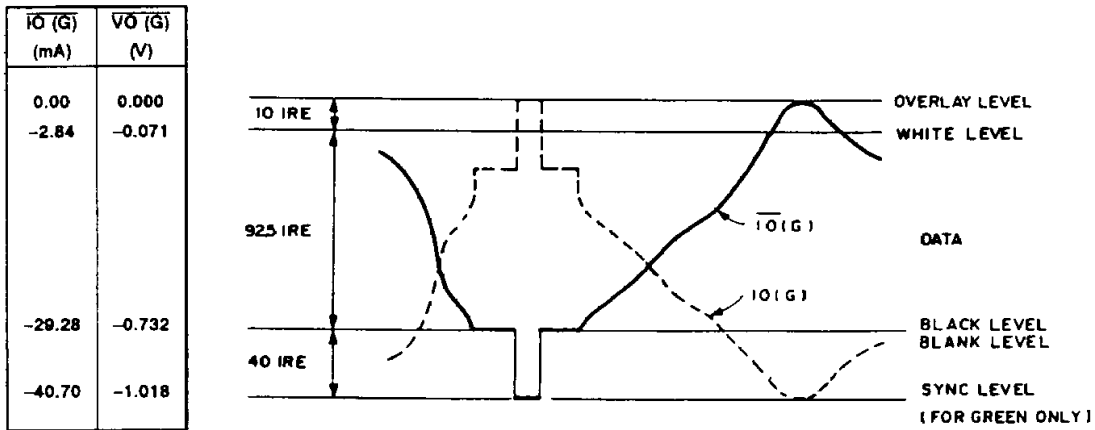
Fig. 3. Composite Video Output Level (GREEN)
