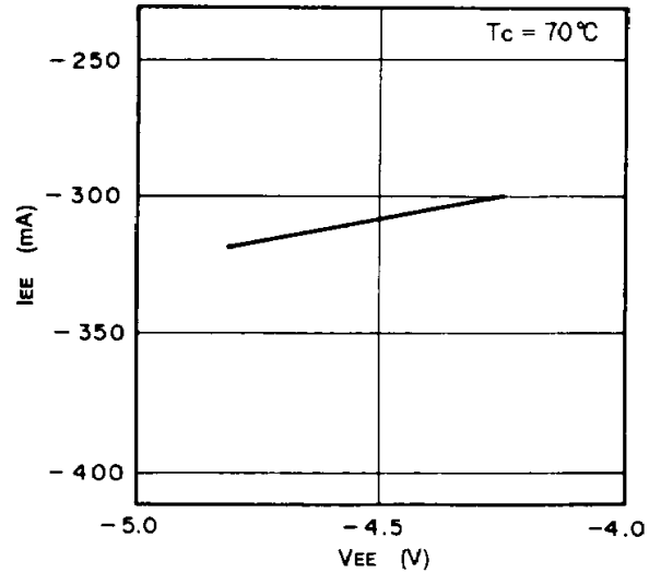
Power supply current vs. Supply voltage
