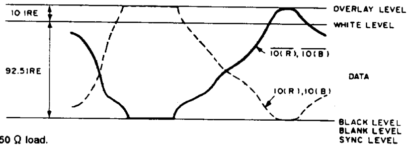
Fig. 4. Composite Video Output Level (RED, BLUE)
