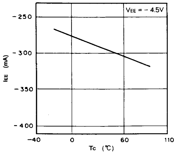
Power supply current vs. T_c
