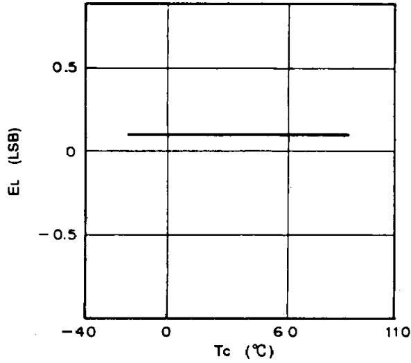
Differential linearity error vs. T_c
