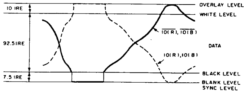
Fig. 2. Composite Video Output Level (RED, BLUE)
