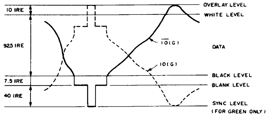
Fig. 1. Composite Video Output Level (GREEN)
