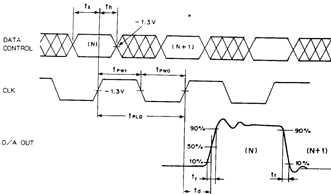
Timing Diagram
