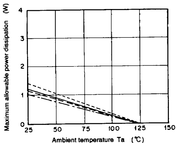
(a) In Still Air
