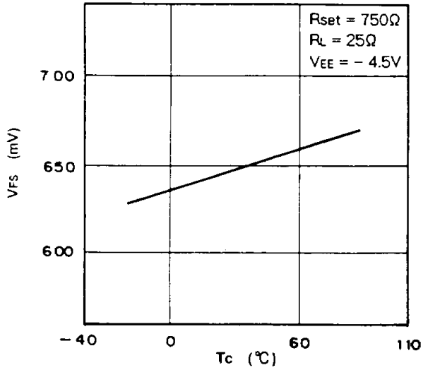
Full gray scale balance vs. T_c
