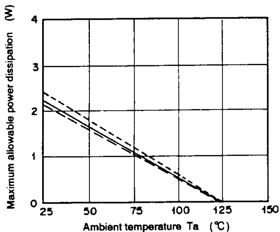
(c) Air Flow Rate 3.0m/sec
