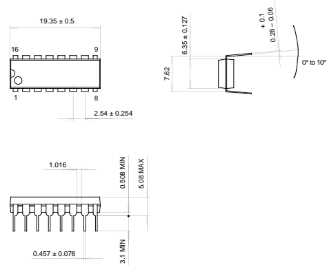
16PIN DIP (PLASTIC) 300mil
