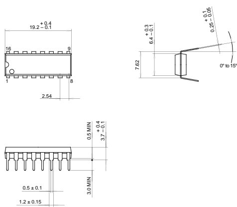
16PIN DIP (PLASTIC) 300mil
