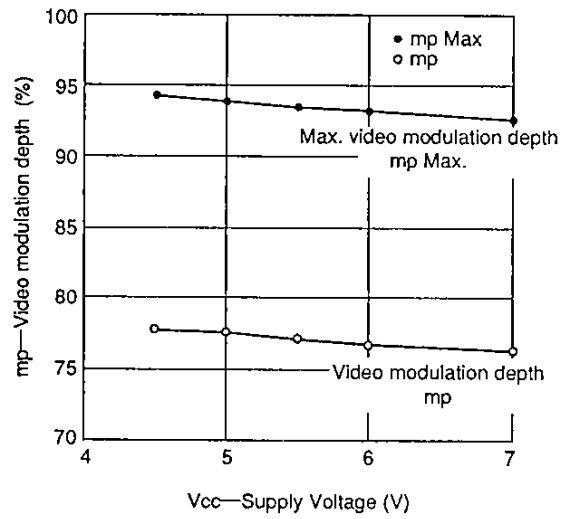
Supply voltage vs. Video modulation depth
