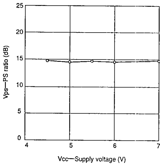
Supply voltage vs. PS ratio
