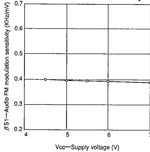
Supply voltage vs. Audio FM modulation sensitivity
