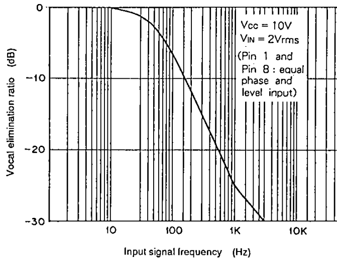
CXA1642 Vocal Elimination Ratio
