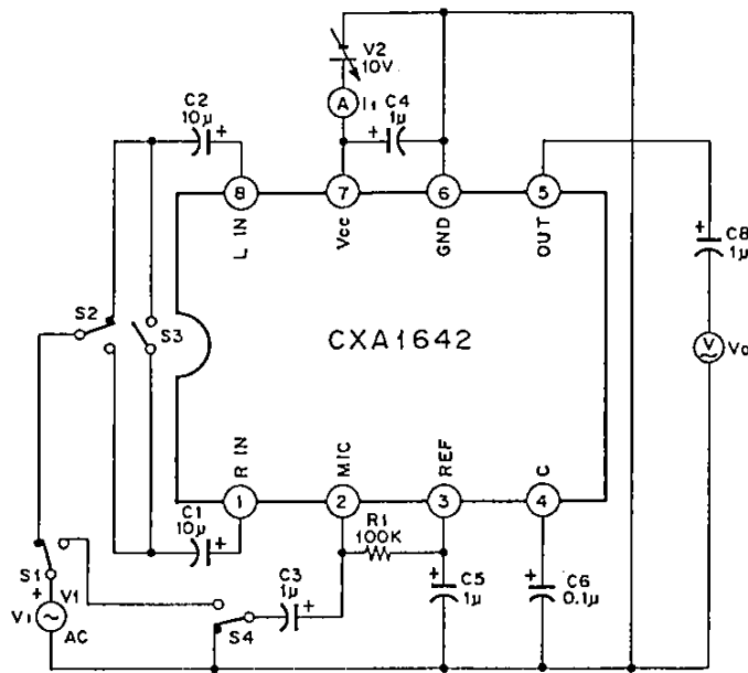
CXA1642 Vocal Elimination Ratio
