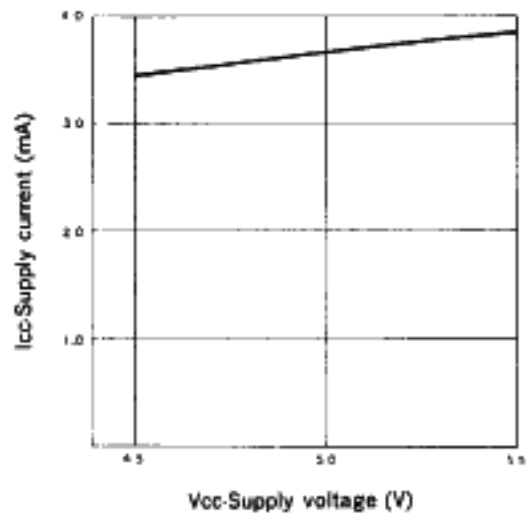
Supply current vs. Supply voltage ( SW=MOD= \text{"High"} , T_a=25^\circ C )
