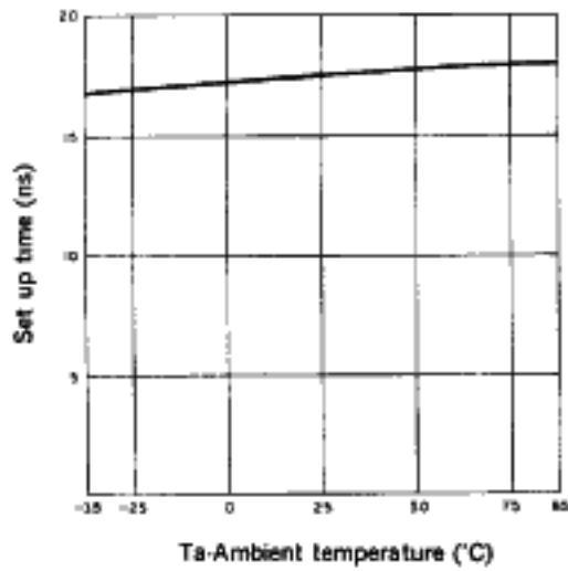
Set up time vs. temperature ( V_{CC}=5V )
