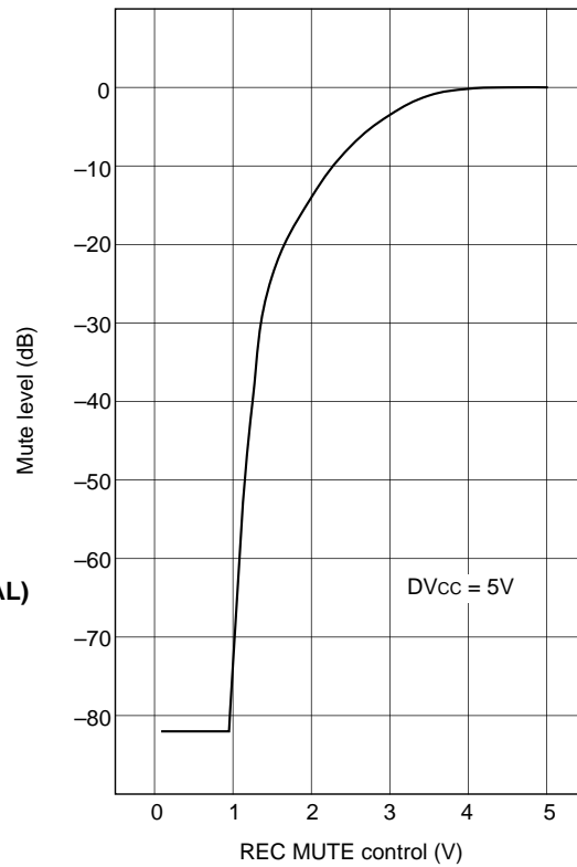
REC MUTE characteristics
