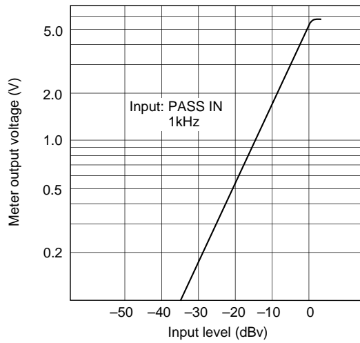
Level meter output characteristics
