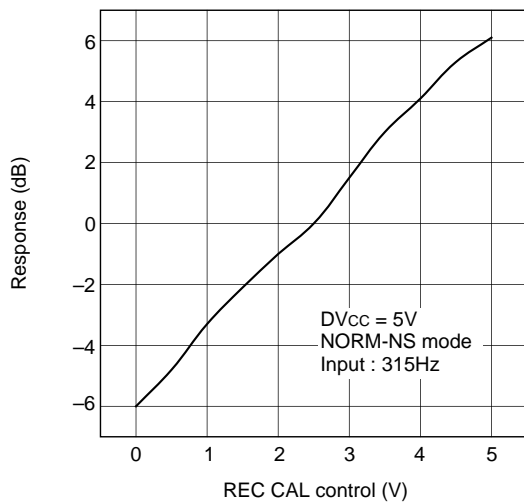
Recording equalizer calibration characteristics (REC CAL)
