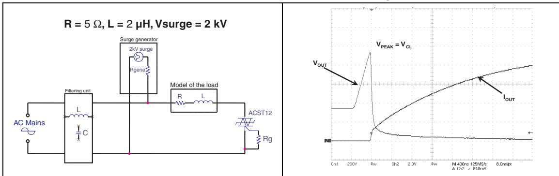
Figure 18. Overvoltage ruggedness test circuit for resistive and inductive loads for IEC 61000-4-5 standards Figure 19. Typical current and voltage waveforms across the ACST12 during IEC 61000-4-5 standard test
