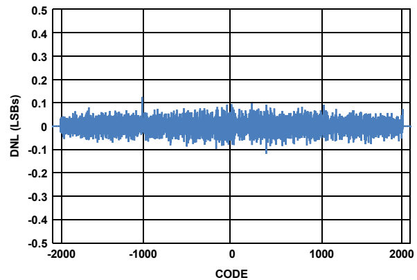
DIFFERENTIAL NONLINEARITY (DNL) vs CODE
