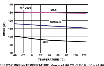
EL8170 CMRR vs TEMPERATURE, V_{CM} = +2.5V TO -2.5V , V_+ , V_- = \pm 2.5V
